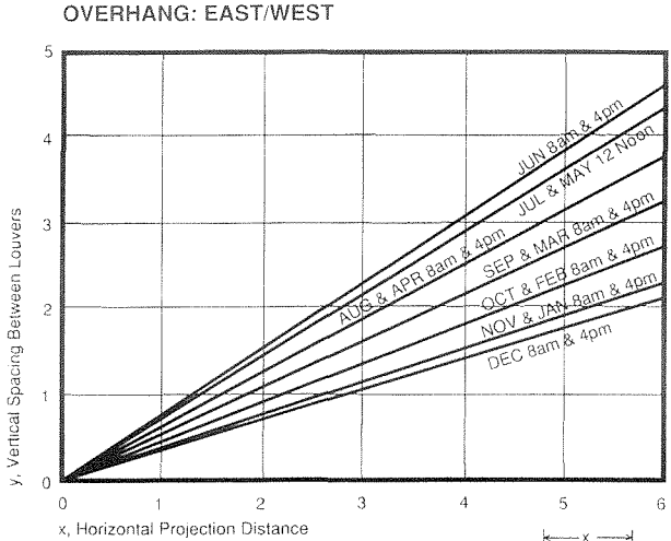
C.4 Required overhang length to shade an east or west window at 21 degrees north latitude between 8:00 a.m. and 4:00 p.m. Length calculated for the 21st day of each month. Calculations by Phil Haisley, AIA.
