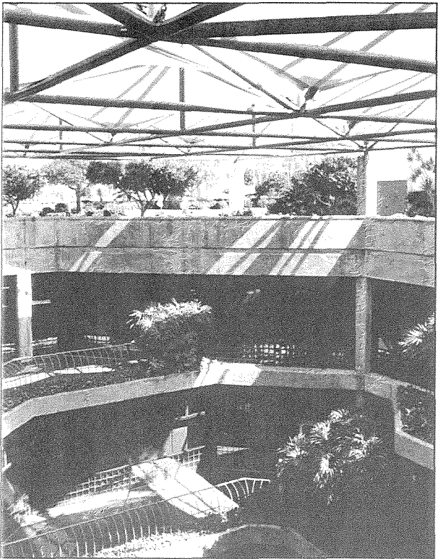
1.5 Detail of light shelf and shading devices on the HMSA Center.
