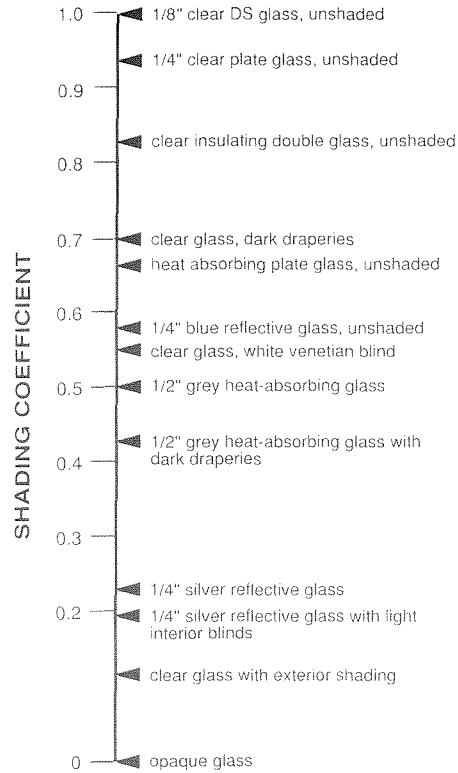
G.3 Shading coefficients for various glass types. Typical shading coefficients vary by manufacturer. Source: Lord.
