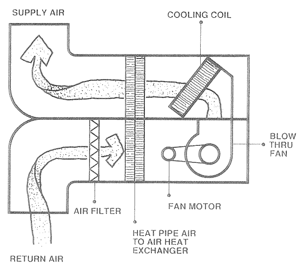
H.5 A heat pipe heat exchanger can reduce humidity in an air-conditioning system using only additional fan energy.
