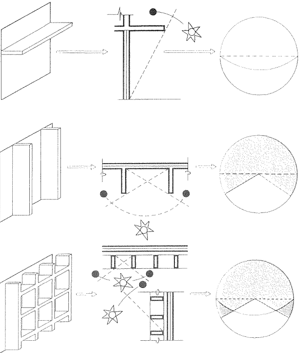
C.2 Overhangs, fins and eggbeaters. Source: Olgyay.
