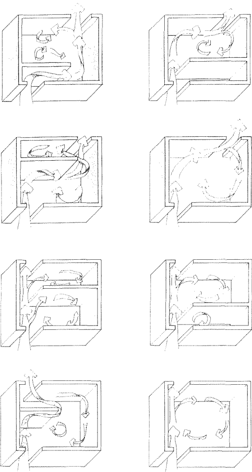
E.15 Air flow patterns with internal partitions.
