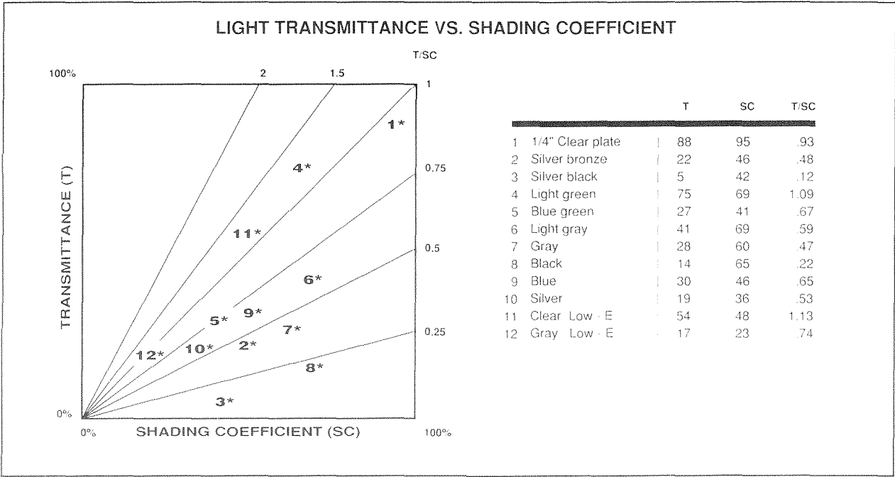
G.4 Light transmittance vs shading coefficient for various glass types. Source: Schiller.
