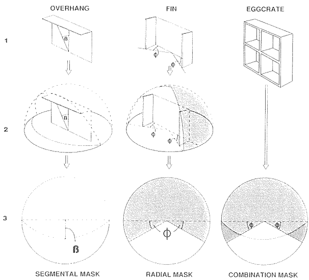
C.7 Construction of a shading mask onto a sun path diagram. Source After Olgyay
