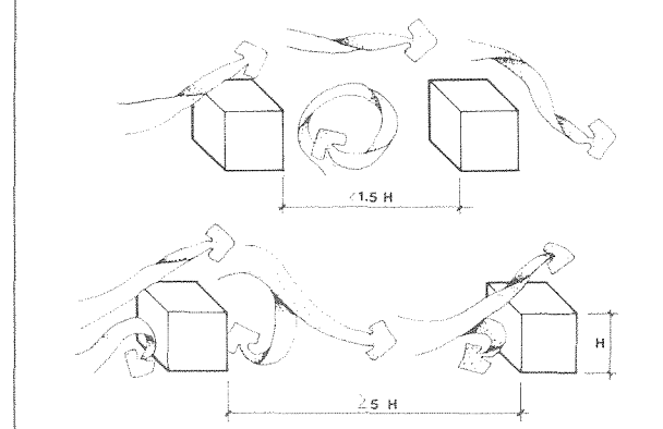
E.4 BUILDING SPACING FOR NATURAL VENTILATION
