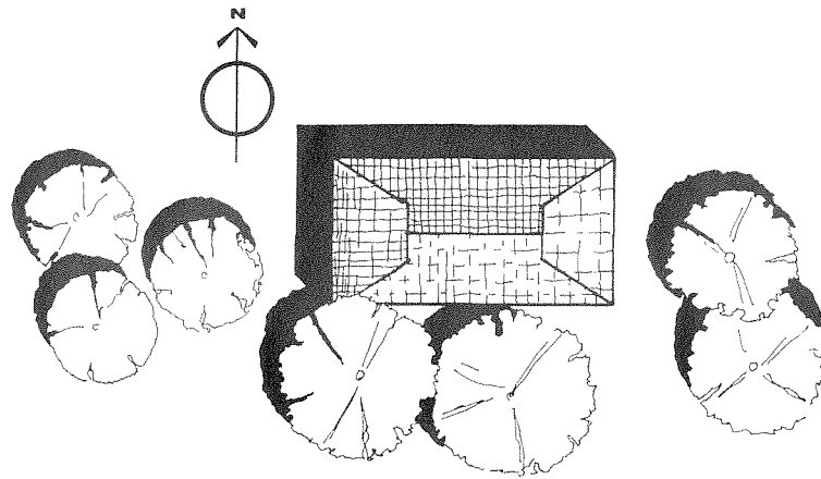
F.2 Landscape locations for shading
