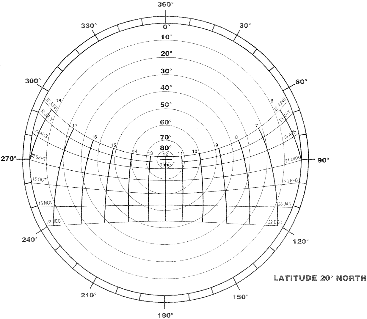
A.17 Sun path diagram for 20° north latitude.
