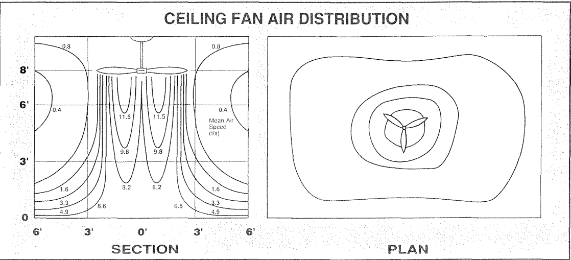
E.16 Air distribution patterns for ceiling fans.
