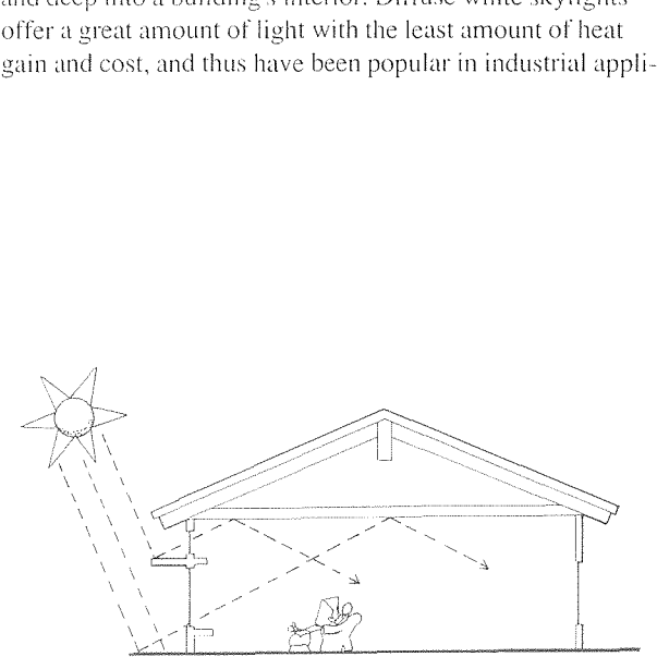
D.6 Bounce daylight off surrounding surfaces to soften and spread it. Source: Evans
