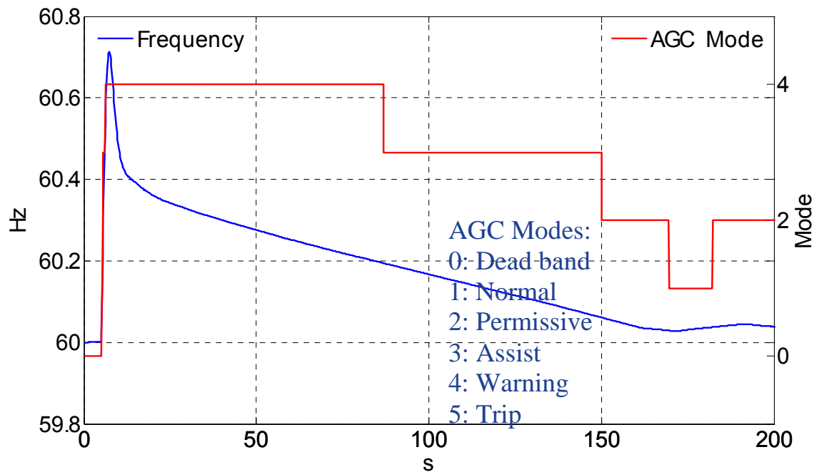
Figure 5-8 System Frequency Response without “Once in a while” ramp rates in AGC
