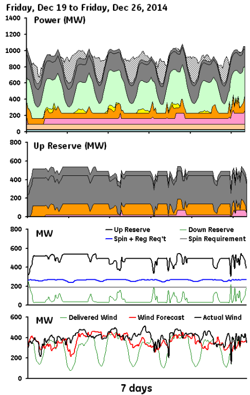
Figure 6-20. Scenario 5B and 3B. Hourly generation, system reserves, and wind profile for two different weeks in 2014, the future study year
