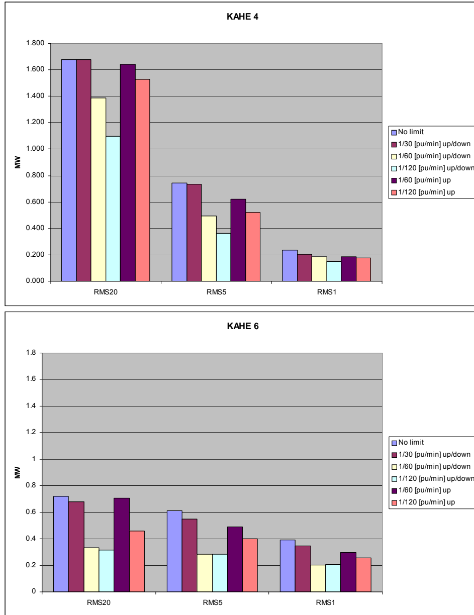
Figure 8-40. Effect of ramp rate limits on Kahe 4 and Kahe 6
