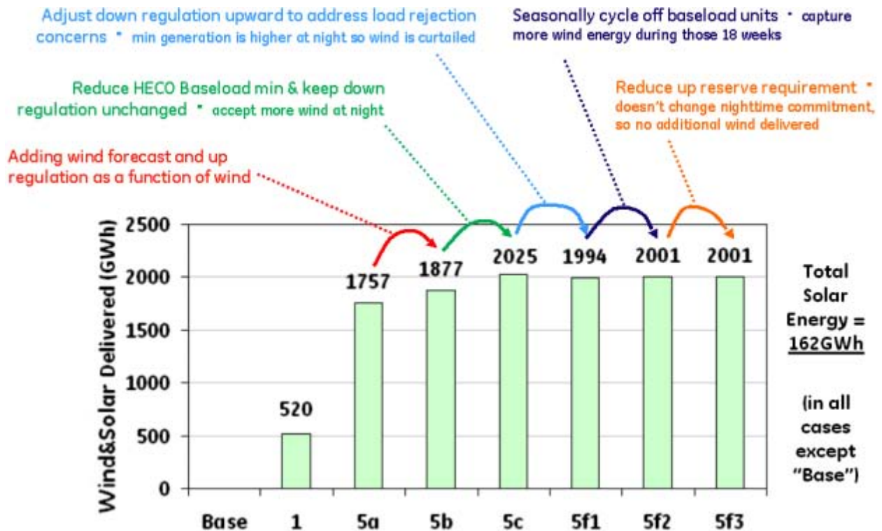
Figure 7-18. Renewable energy delivered under different scenarios
