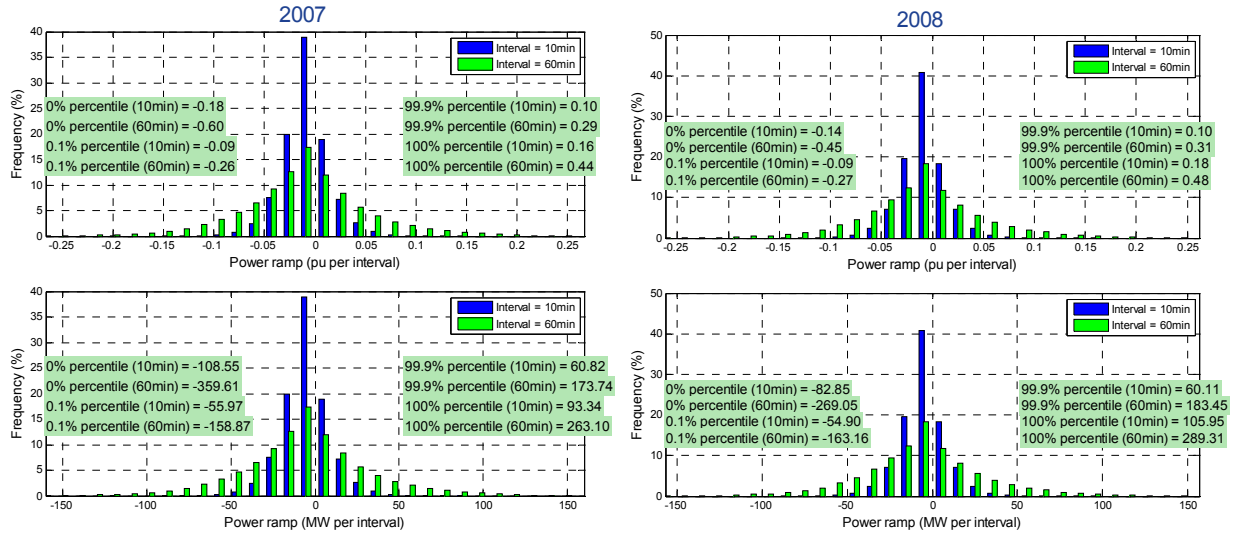
Figure 6-4. Wind and solar power variability for Scenario 5 (2007 on left, 2008 on right)
