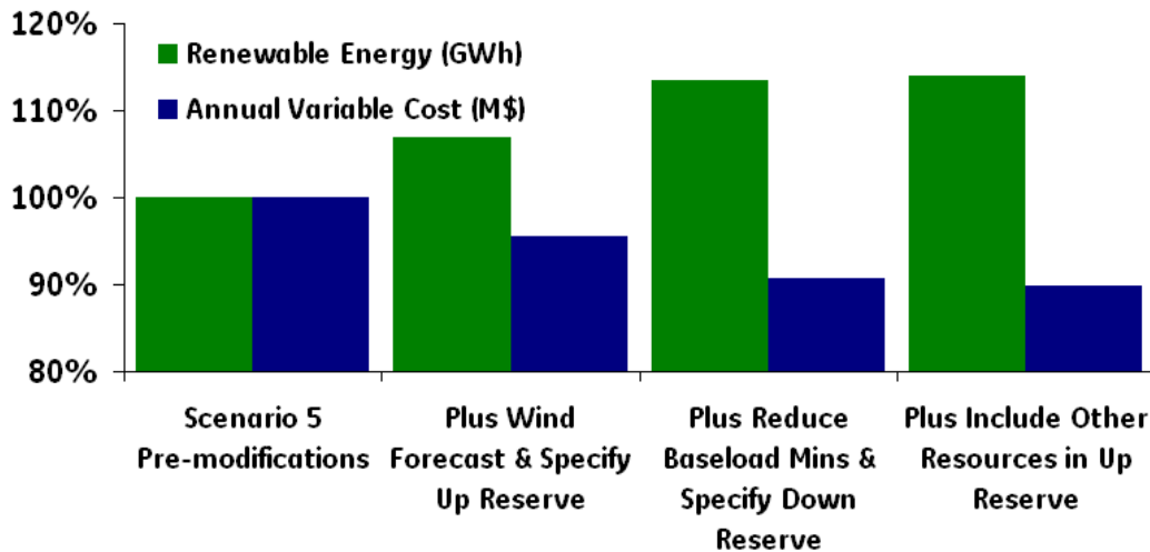
Figure 1-9. Scenario 5. Reduction in variable cost and increase in wind and solar energy delivered for staged strategies.
