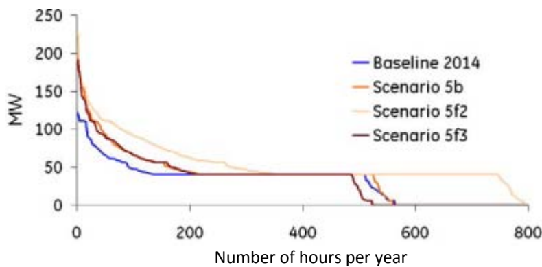
Figure 7-16. Scenario 5F3. Duration curve of fast-starting power from fast-starting units
