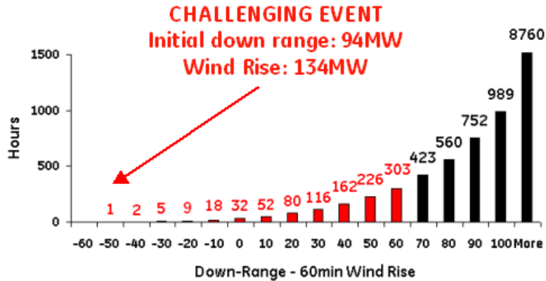
Figure 8-16. Challenging events in the 60 minute screening (Scenario 5F3)
