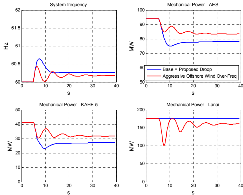
Figure 8-46: PSLF transient simulation result for 80 MW load rejection (Sc 5F3, aggressive offshore wind plants over frequency control)
