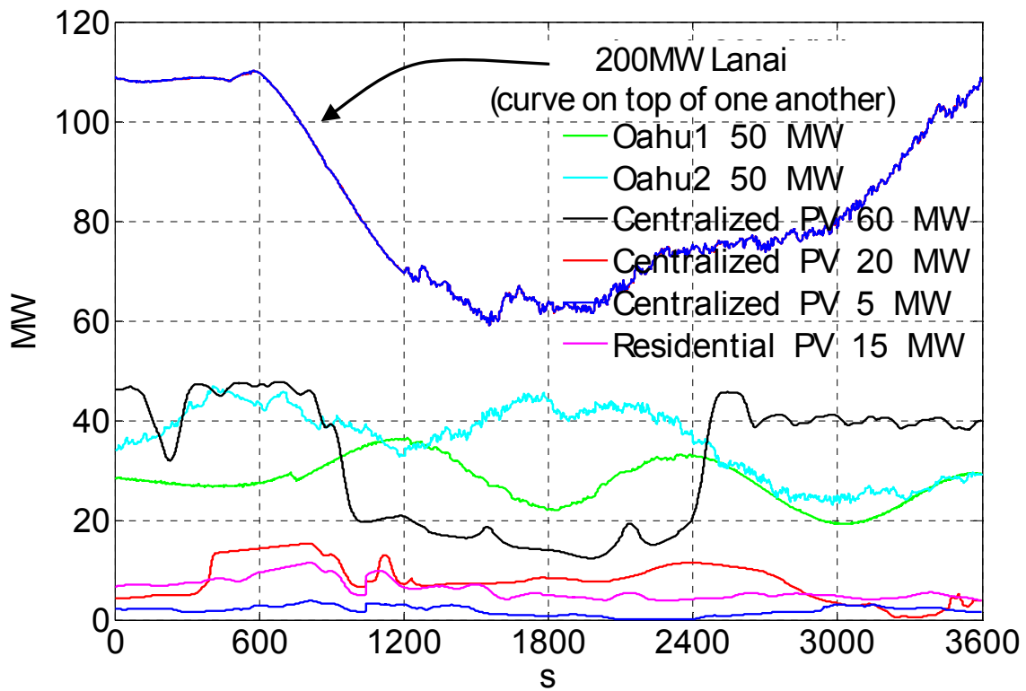
Figure 8-11. Hour 6851 wind and coherent solar power variability for Scenario 3F3
