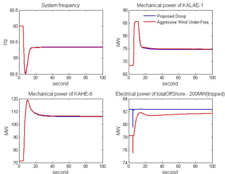
Figure 8-50: Transient simulation result for 200 MW cable trip for scenario 5F3. Aggressive wind under-frequency control. Base case (blue) and wind plant control case (red). The bottom right figure shows the un-tripped off-island wind plant carrying ~4 MW of up-reserve. All cases, including the base case, assume future droop settings for thermal units.
