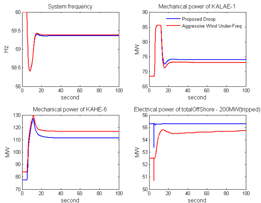
Figure 8-53: Transient simulation result for 200 MW cable trip for scenario 3F3. Aggressive wind under-frequency control. Base case (blue) and wind plant control case (red). The bottom right figure shows the un-tripped off-island wind plant carrying approximately 4 MW of up-reserve. All cases assume future droop settings.
