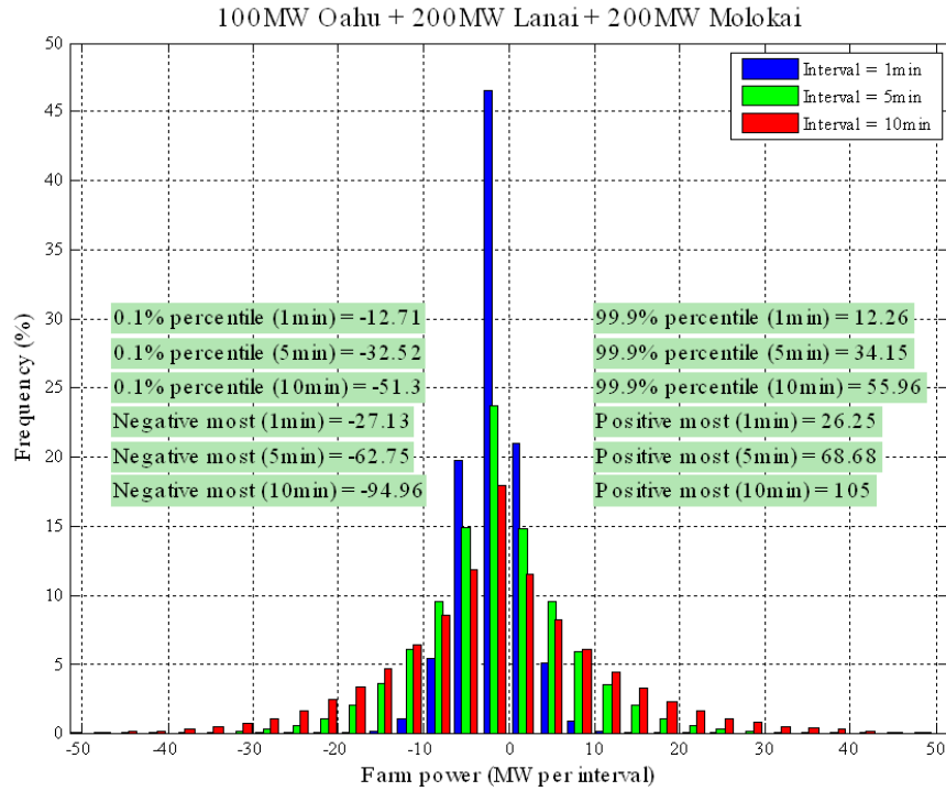
Figure 6-5. Histogram of wind power variation at 1 minute, 5 minute, and 10 minute interval for 2007 and 2008 wind power data.
