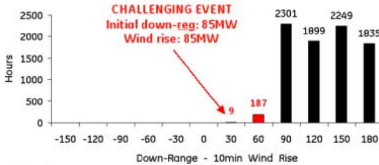
Figure 8-19. A challenging event in the 10 minute screening (Scenario 5F3)
