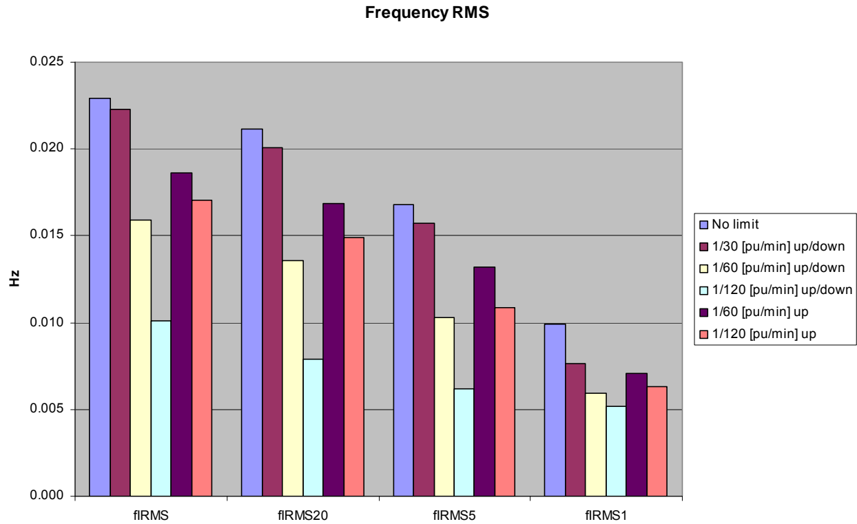
Figure 8-39. Effect of ramp rate limits on system frequency
