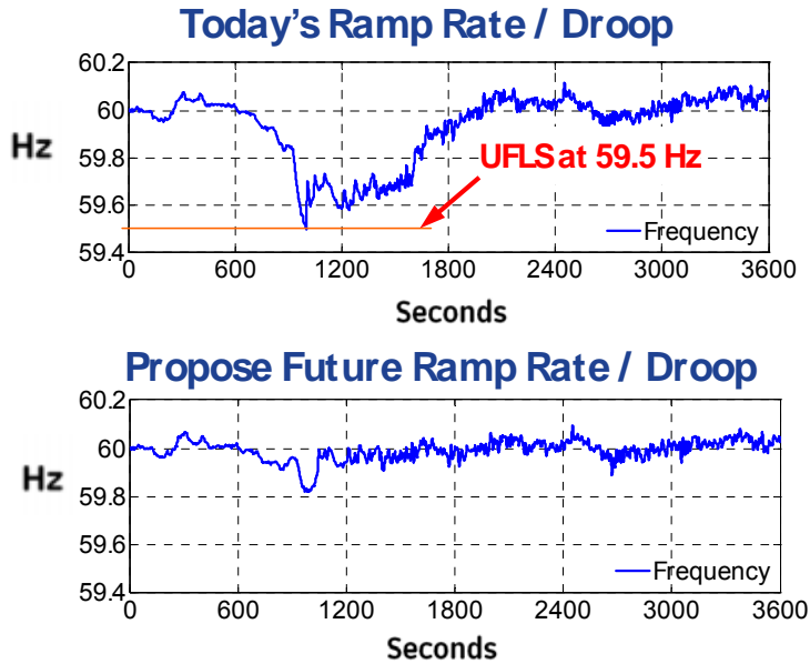
Figure 1-12. Large wind, solar, load change over 10 minute that challenged the system ramp rate capability
