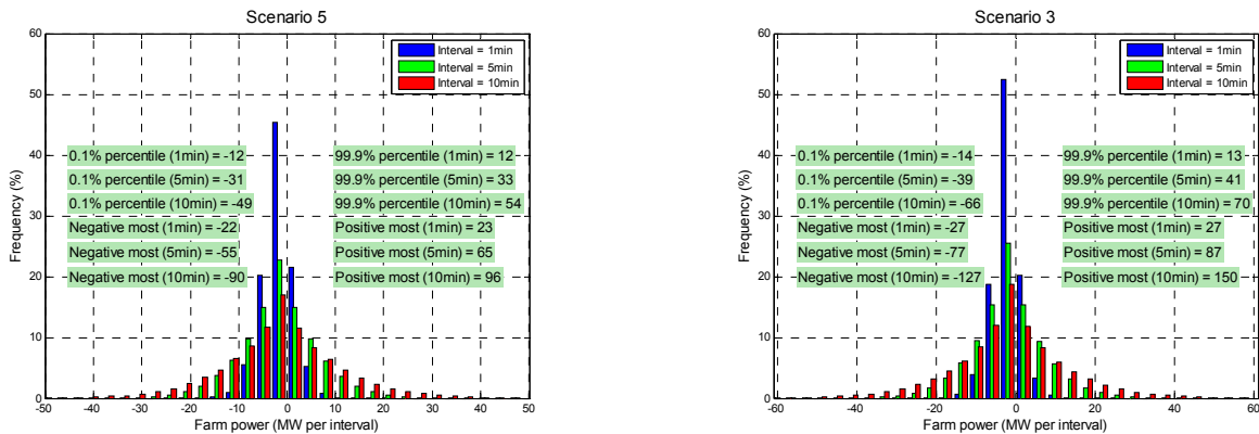
Figure 8-10. Short-timescale wind variability in Scenario 3 and Scenario 5
