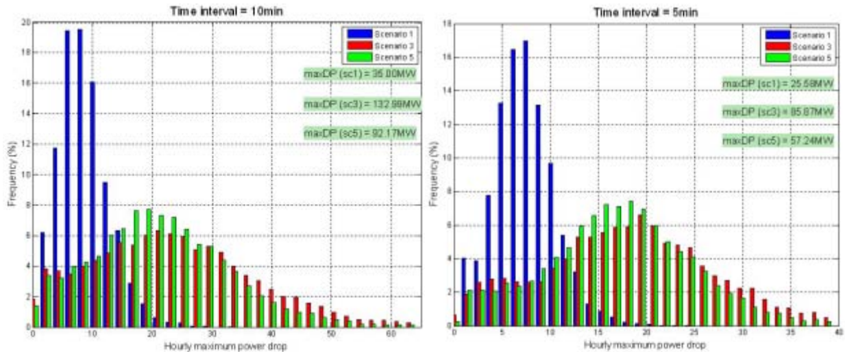
Figure 6-6. Histogram of wind power drops for each hour of the year (2007 wind data, reducing off-island wind power by 5% due to HVDC losses). No solar power changes are considered.
