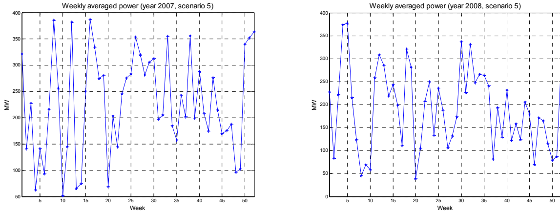
Figure 7-8. Average weekly wind data for 2007 and 2008
