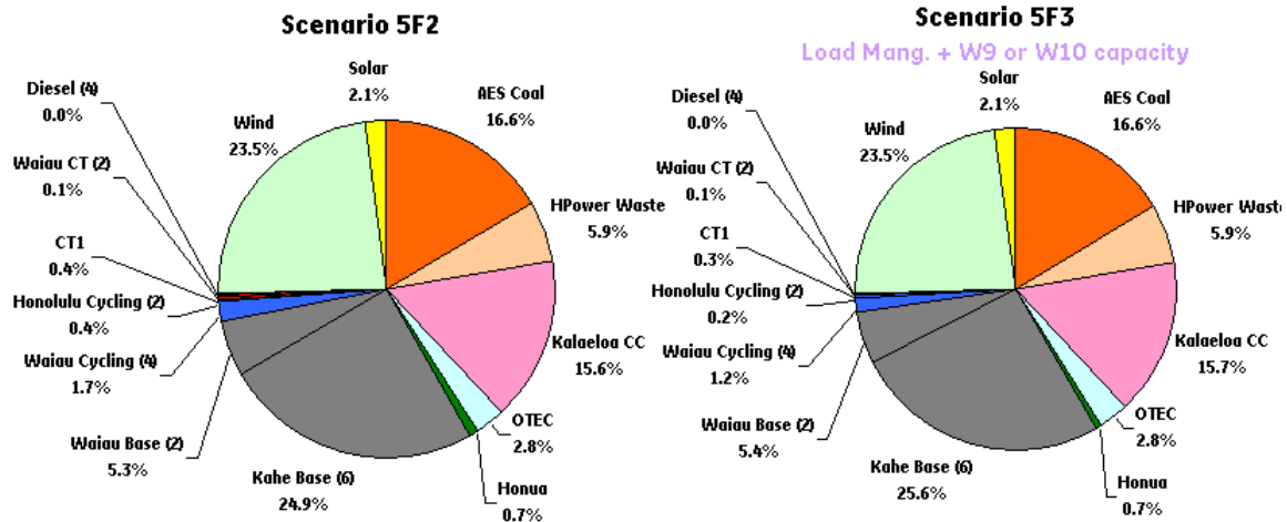
Figure 7-14. Scenario 5F3. Annual energy production by unit type
