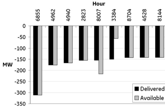
Figure 8-2. Highest drop in wind power for Scenario 5B (available and delivered)
