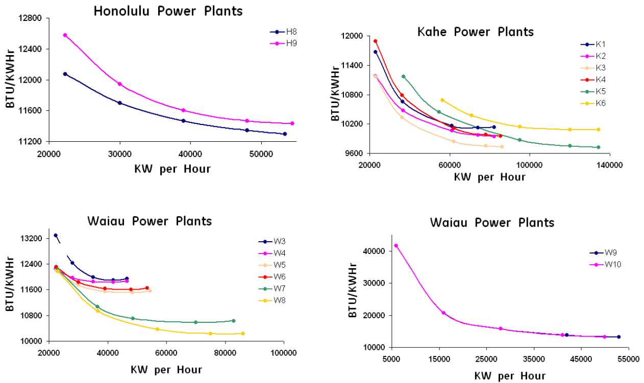
Figure 6-10. Thermal unit heat rates for Baseline 2014
