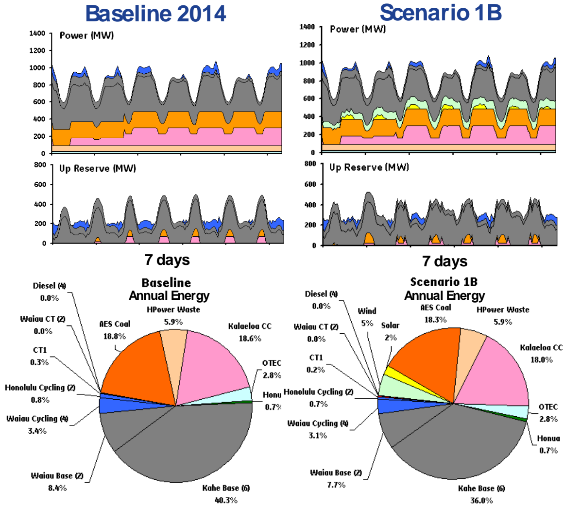
Figure 6-15. GE MAPS™ results for Scenario 1
