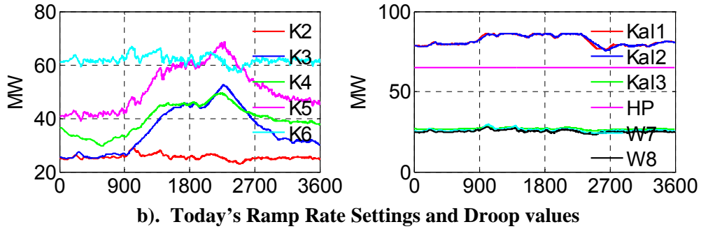
Figure 8-26. Hour 5795 Scenario 5F3 - Generating Unit Response
