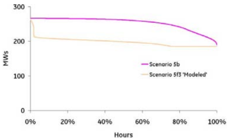
Figure 7-13. Scenario 5F3. Modified regulating reserve requirement in Scenario 5F3 compared to Scenario 5B
