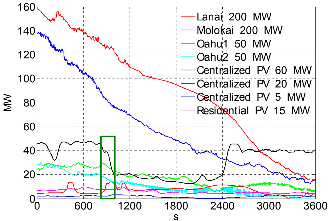
Figure 8-5. Wind and Solar Power Variability for Hour 6855
