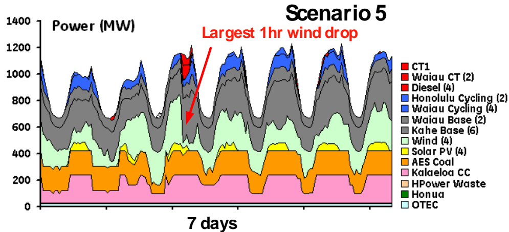
Figure 1-5. An example week of operation for the Oahu power system with 500 MW of wind power and 100 MW of solar power (Scenario 5)
