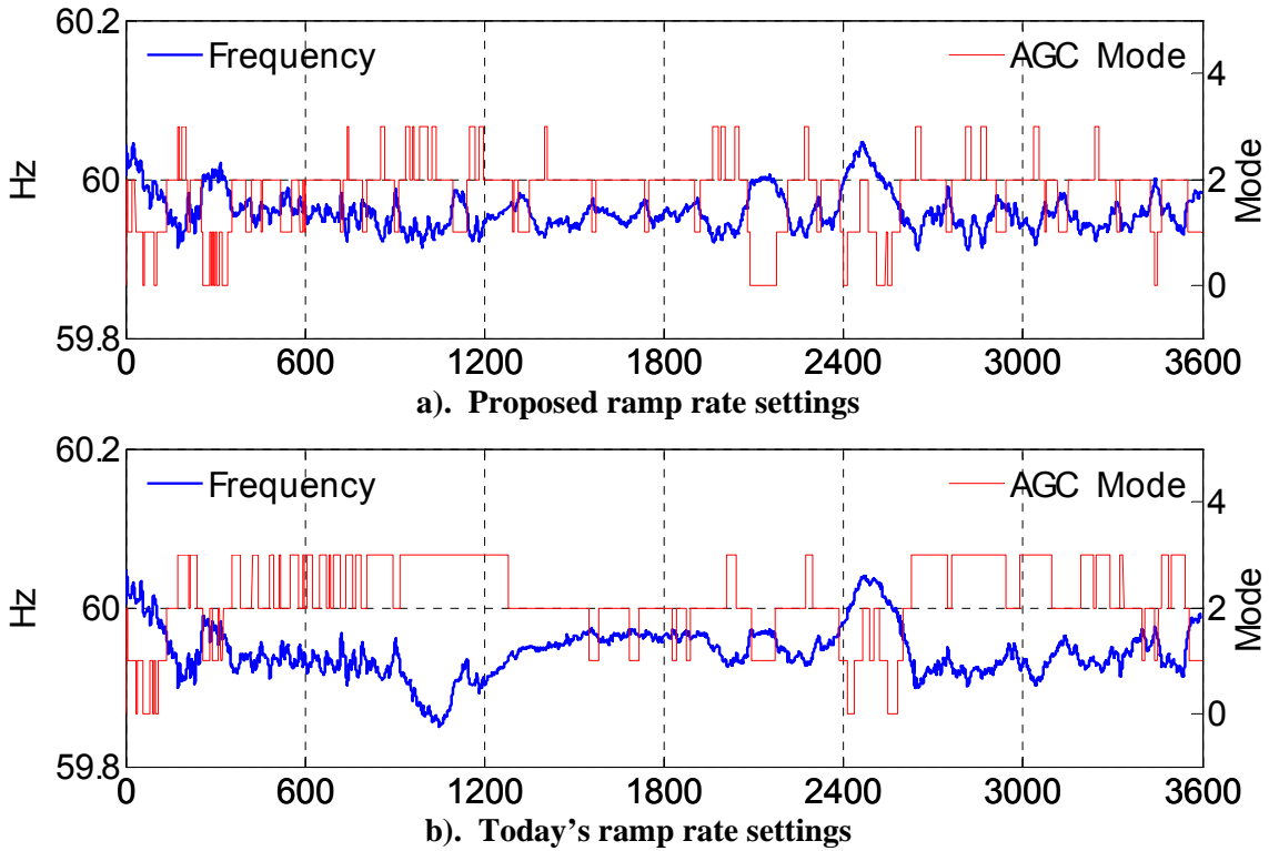
Figure 8-7. Hour 6855 – Frequency response (x-axis in seconds)
