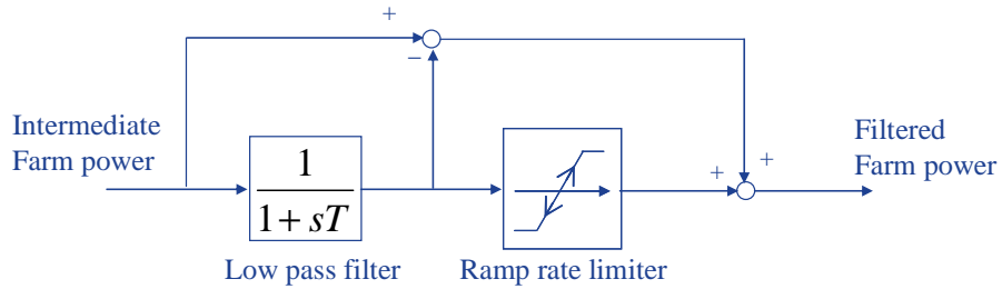
Figure 8-36. Processing filter for ramp rate control
