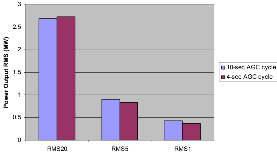
Figure 8-35. AGC cycle sensitivity - maneuvering of HECO units
