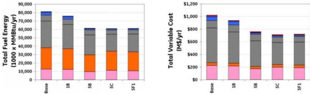
Figure 7-5. Scenario 5F1: Fuel energy and total variable cost of operation
