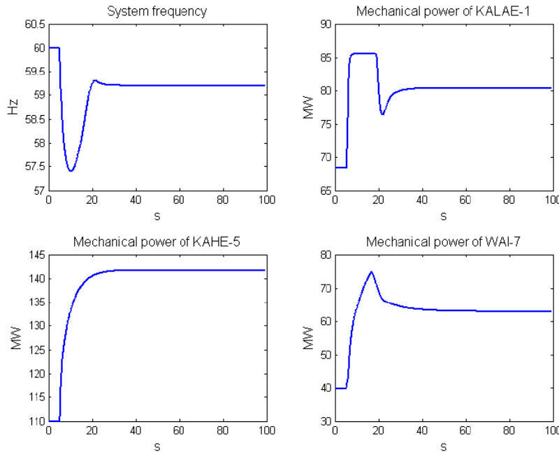
Figure 8-54. Trip of AES in Scenario 1 for future droop settings for thermal units
