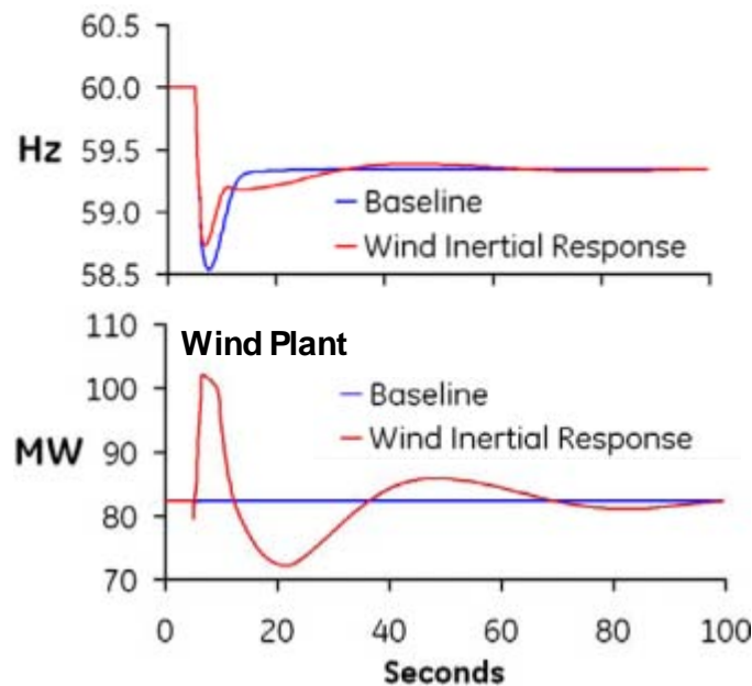
Figure 1-14. 200 MW cable trip event in Scenario 5 with future thermal unit droop characteristics, with and without wind turbine inertial-type response. Second figure shows response from remaining off-island wind plant.
