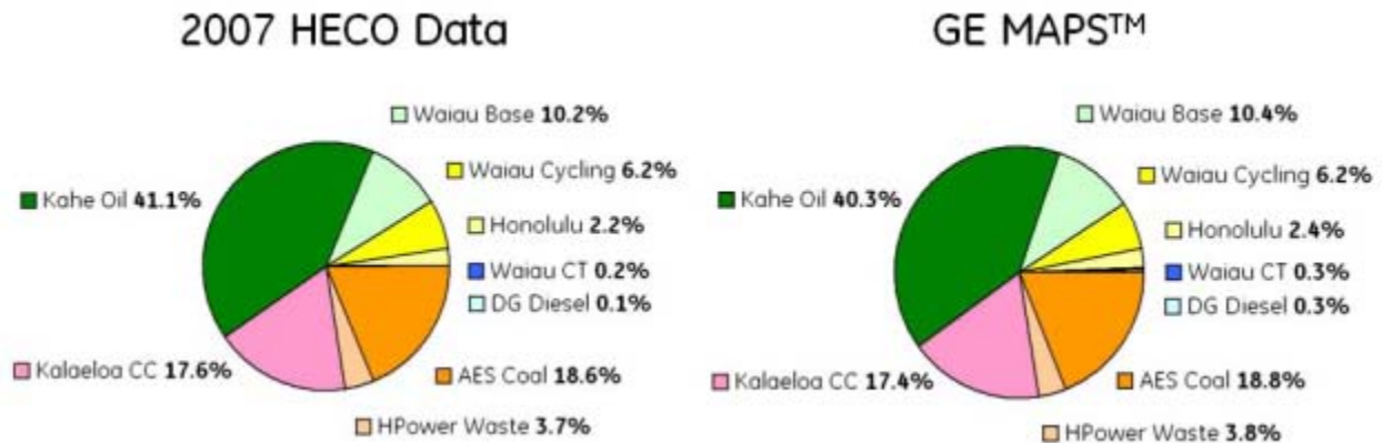
Figure 5-4 Electricity production, by unit type, for 2007.
