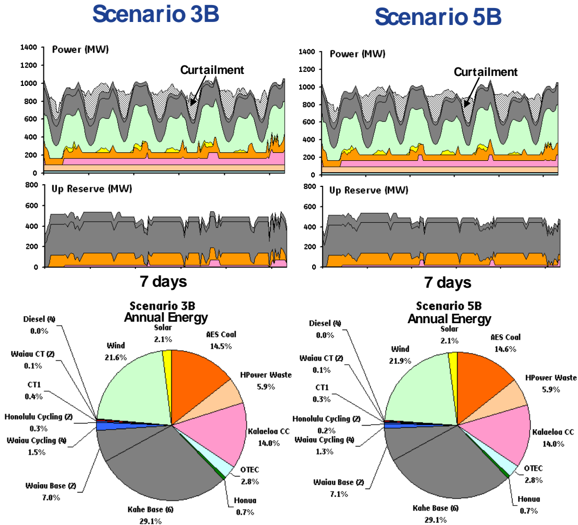
Figure 6-19. Scenario 3: Annual energy production by unit type
