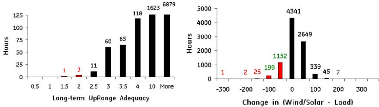
Figure 8-9. Long-term analysis for Scenario 5F3
