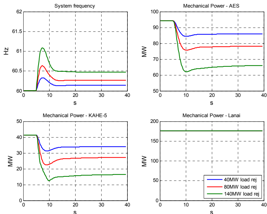
Figure 8-42: PSLF transient simulation result for load rejection (Sc 5F3, base case comparison while setting the minimum valve position of Kahe 5 governor to zero)
