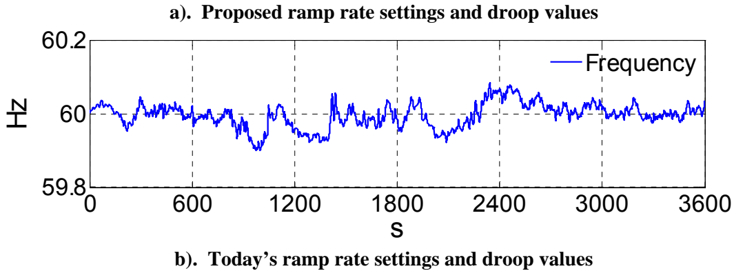
Figure 8-25. Hour 5795 Scenario 5F3 – Frequency Response
