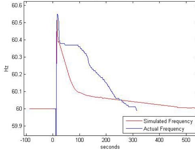
Figure 5-7 Exhibit 12, Scenario 3, Fast AGC Tuning, Simulated vs. Actual Frequency (wide scale)
