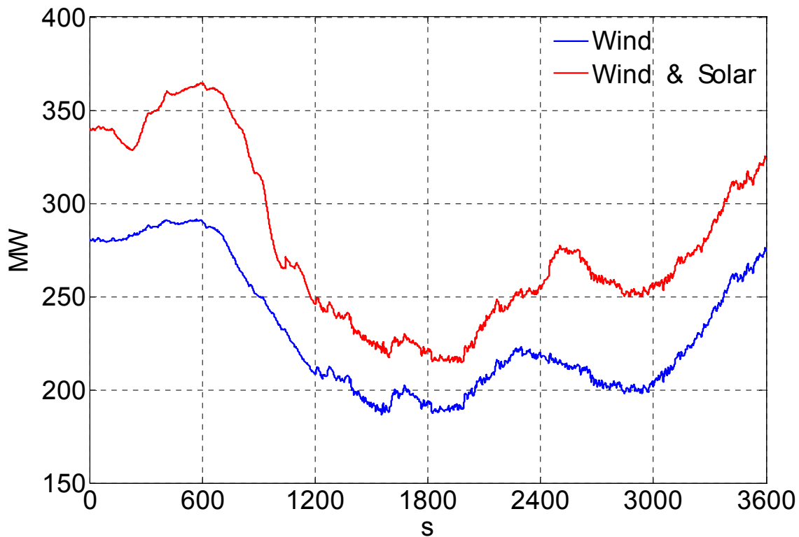
Figure 8-12. Hour 6851 Total Wind and Solar Power Variability
