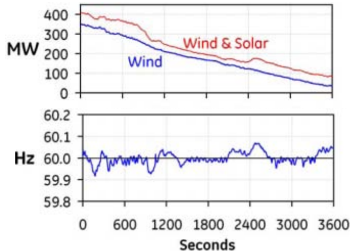
Figure 1-11. Frequency performance during largest 60-minute wind power drop
