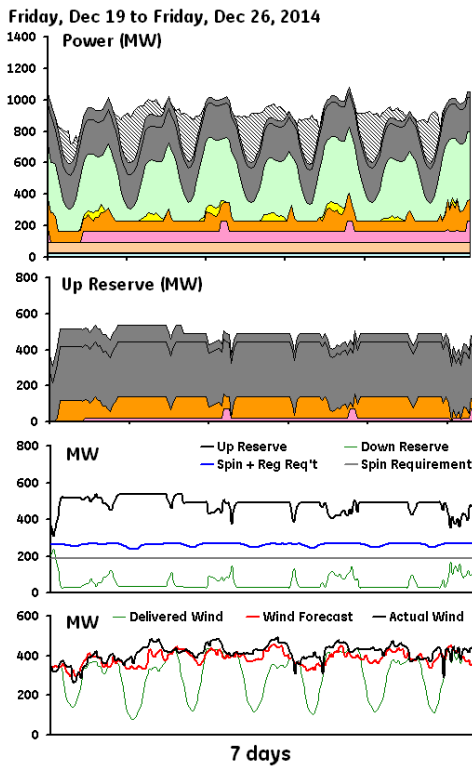
Figure 6-20. Scenario 5B and 3B. Hourly generation, system reserves, and wind profile for two different weeks in 2014, the future study year
