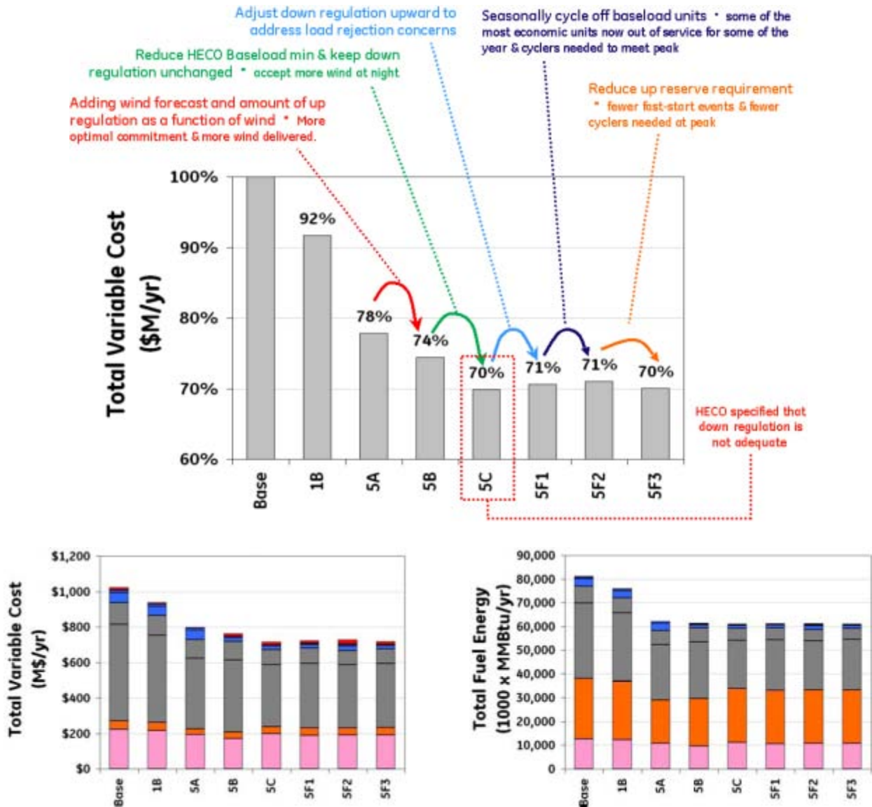
Figure 7-19. Total variable cost of operation and fuel consumption for each scenario
