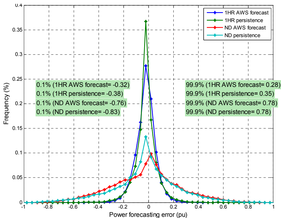
Figure 6-8. Histogram of wind forecasting error (actual power – forecasted power), for two years of data, for 100 MW Oahu + 400 MW Lanai (Scenario 3, excluding solar power). ND = next day.
