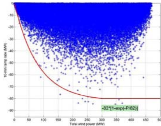
Figure 6-9. Scenario 5: 10 minute drops in wind power as a function of the wind power available at the start of the 10 minute interval. Results based on 2007 and 2008 modeled wind data from AWS Truepower.
