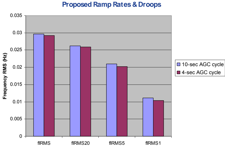
Figure 8-34. AGC cycle sensitivity - Hour 5795 Scenario 5F3
