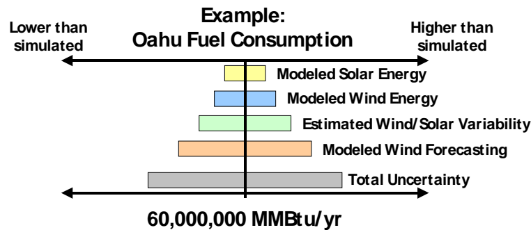
Figure 5-2. Illustration of the cumulative effect of modeling uncertainties and limitations on the annual fuel energy consumption on Oahu
