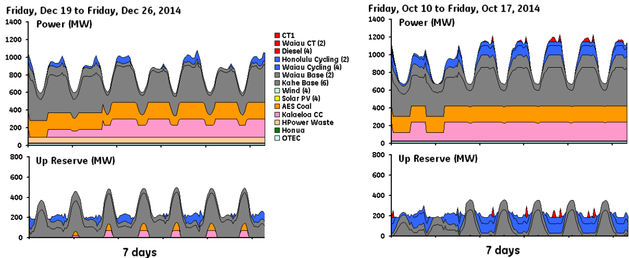
Figure 6-13. Baseline 2014 scenario. Hourly generation for two different weeks.
