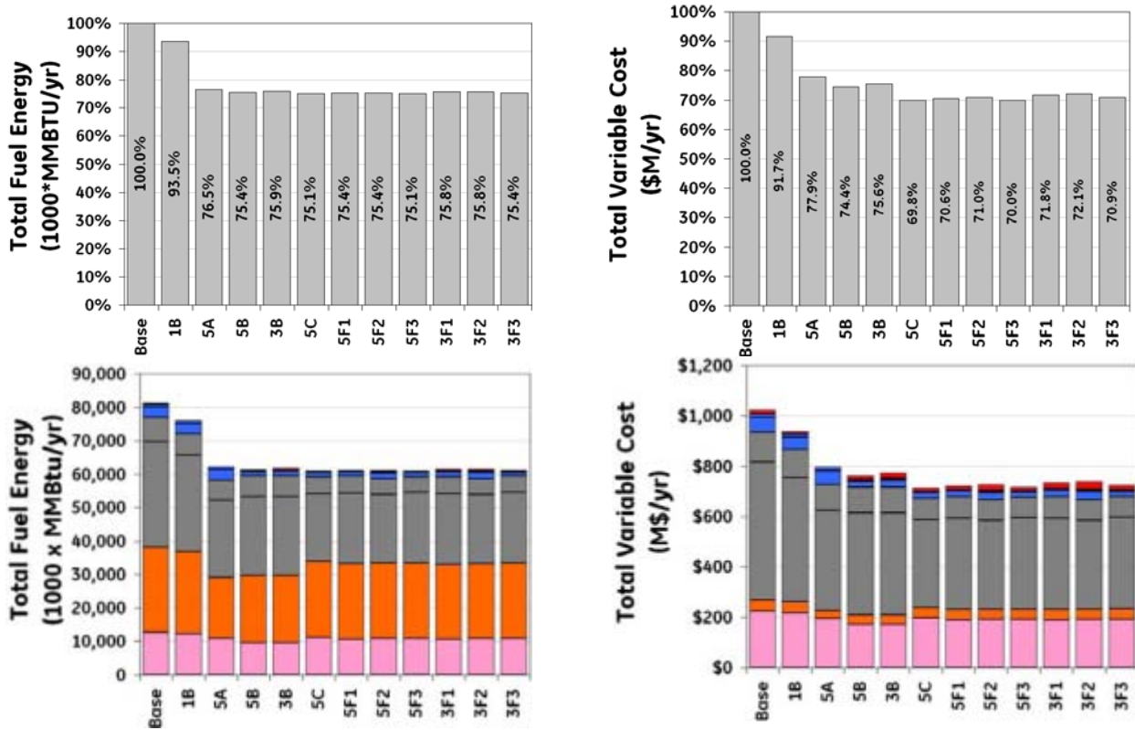
Figure 7-24. Total annual variable cost and fuel consumption for each scenario
