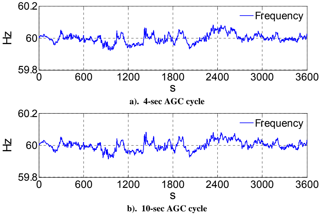
Figure 8-32. Hour 5795 Scenario 5F3 – Frequency Response
