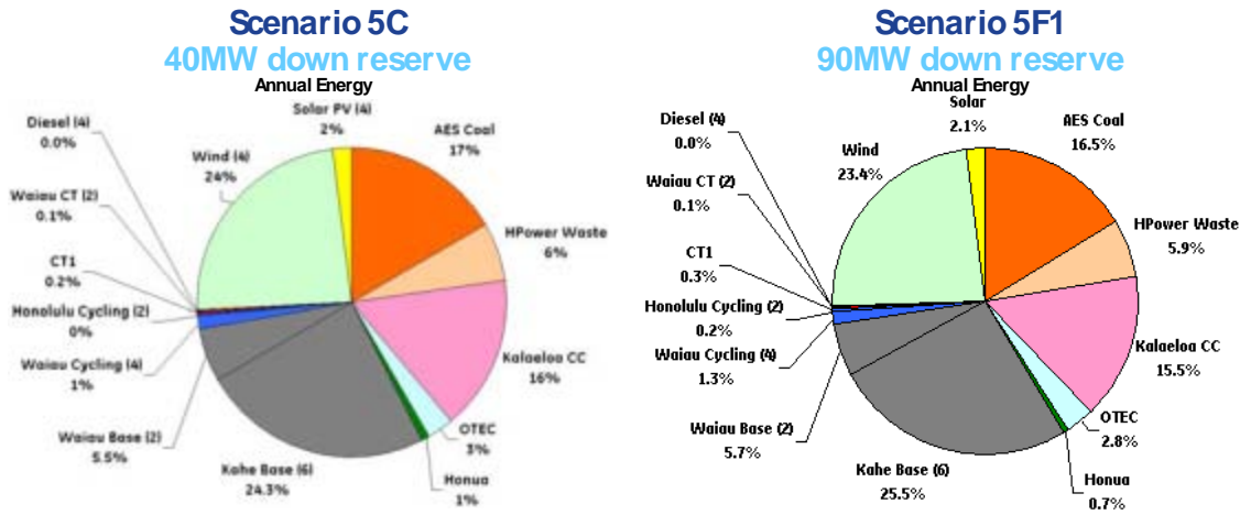
Figure 7-4. Scenario 5F1. Annual energy production by unit type
