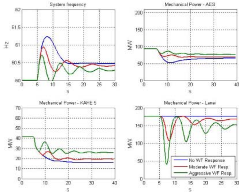
Figure 8-47. 140 MW load rejection event for all with plants in Scenario 5F3: No wind plant over-frequency control, moderate wind plant over-frequency control and aggressive wind plant over-frequency control. All cases assume future droop settings for thermal units.
