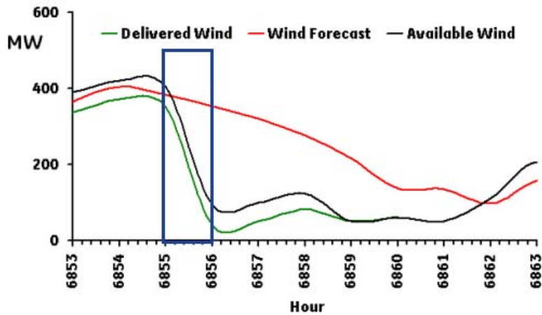
Figure 8-3. Forecasting error for the Hour 6855
