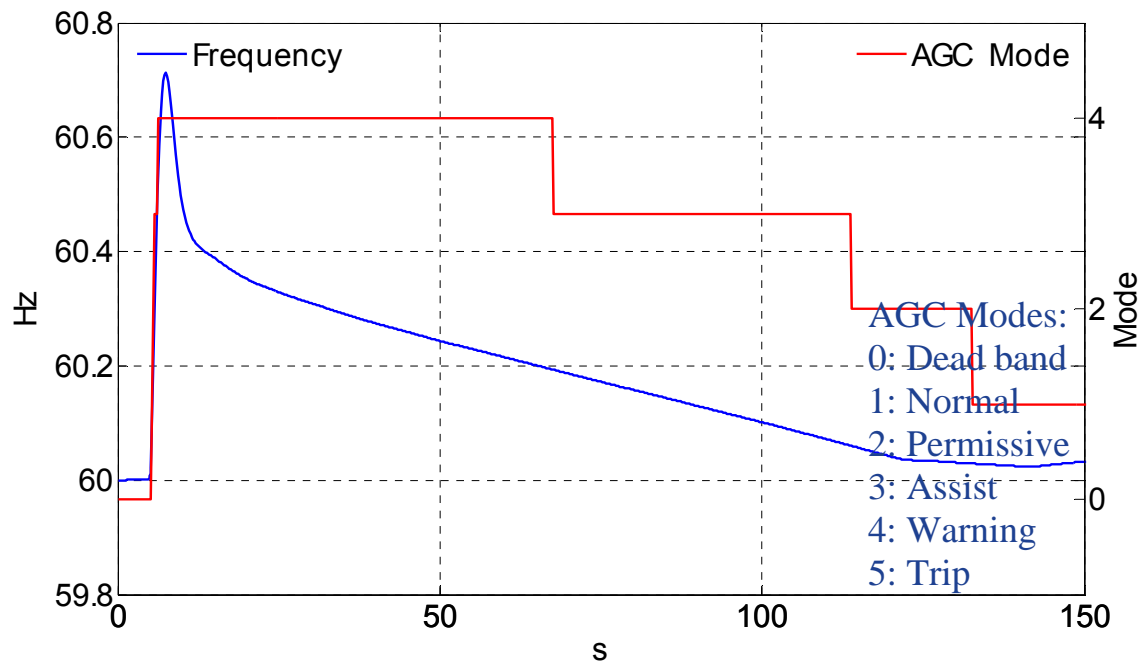
Figure 5-9 System Frequency Response with “Once in a while” ramp rates in AGC
