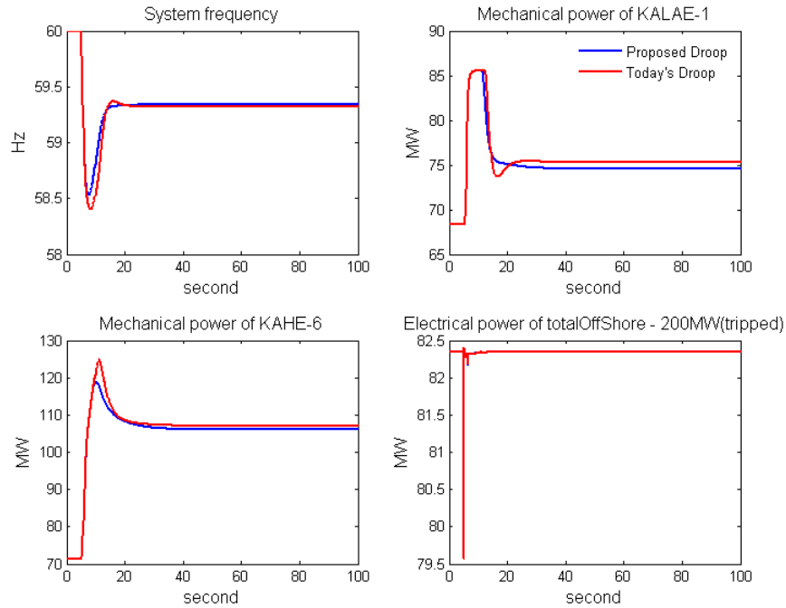
Figure 8-48: Transient simulation result for 200 MW cable trip for scenario 5F3. Sensitivity to thermal unit droop. Proposed droop (blue) and today's droop (red)
