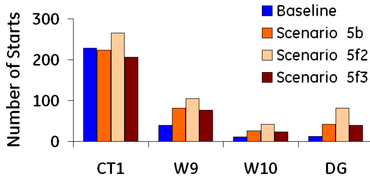
Figure 7-15. Scenario 5F3. Number of fast-start events by unit. Note that the number of fast-start events for the four Airport DGs are added together.
