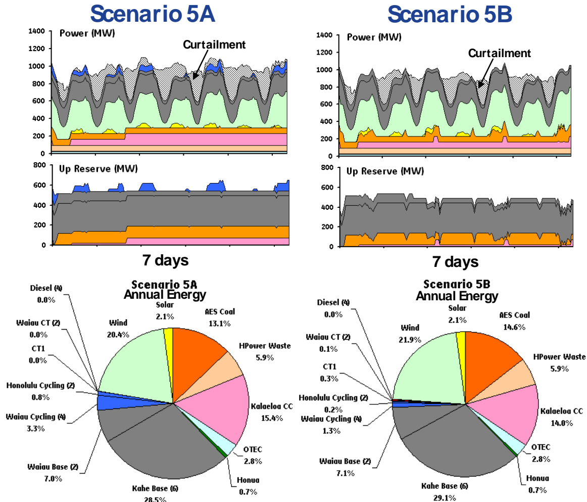
Figure 6-16. Scenario 5: One week of generation and annual energy production by unit type
