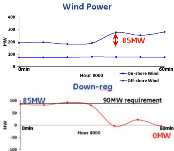
Figure 8-20. A challenging 10 minute event in Scenario 5F3
