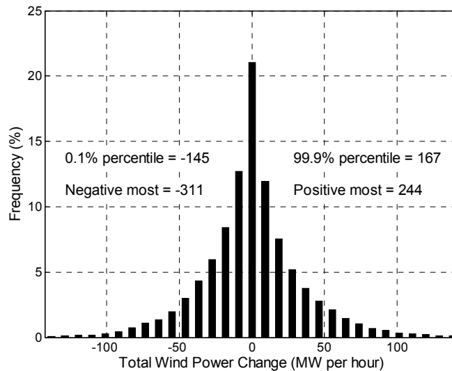
Figure 1-10. Histogram of total wind power changes over 60-minute for Scenario 5 for the wind energy delivered to the Oahu system (two years of simulated wind power data from AWS Truepower).
