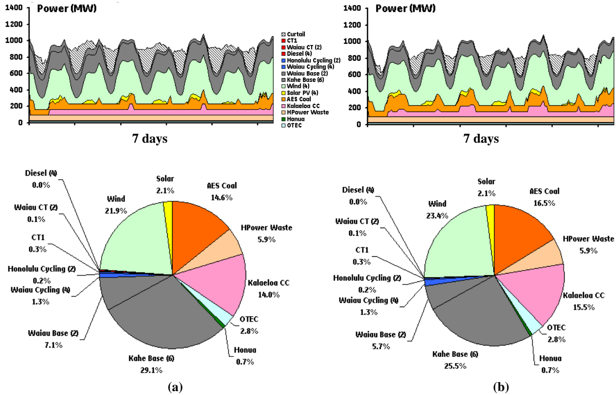
Figure 7-28. Impact of reducing the minimum operating power of 7 HECO baseload units and increasing the down-reserve requirement from ~40 MW to ~90 MW. Comparison of seven days of production during the week of highest available wind power and annual energy production for: (a) Scenario 5 + Strategy #1, and (b) Scenario + Strategy #1 and #2
