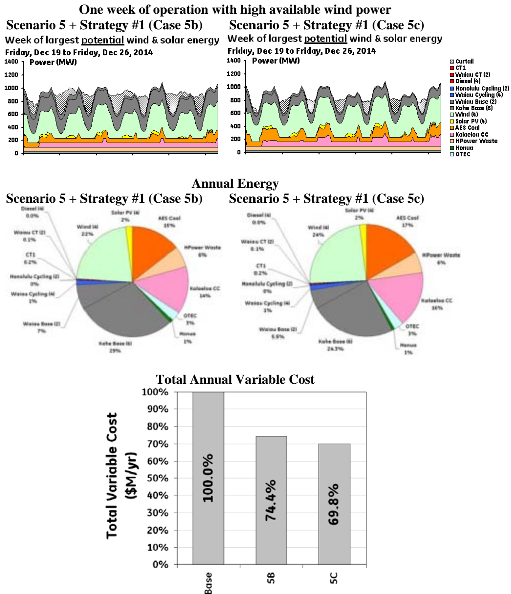
Figure 7-27. Summary of total variable cost savings and energy
