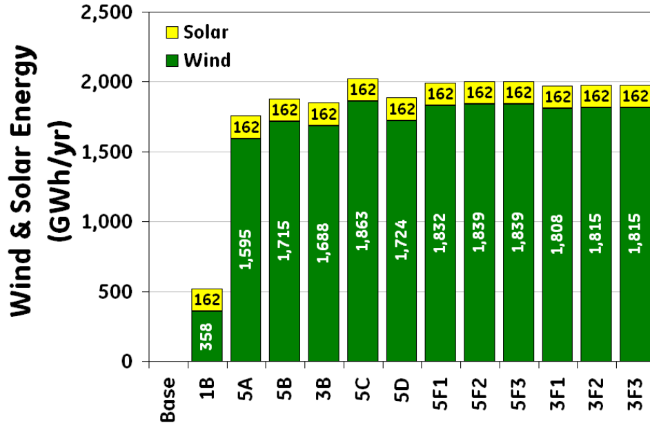
Figure 7-23. Delivered wind energy plus solar energy for each scenario
