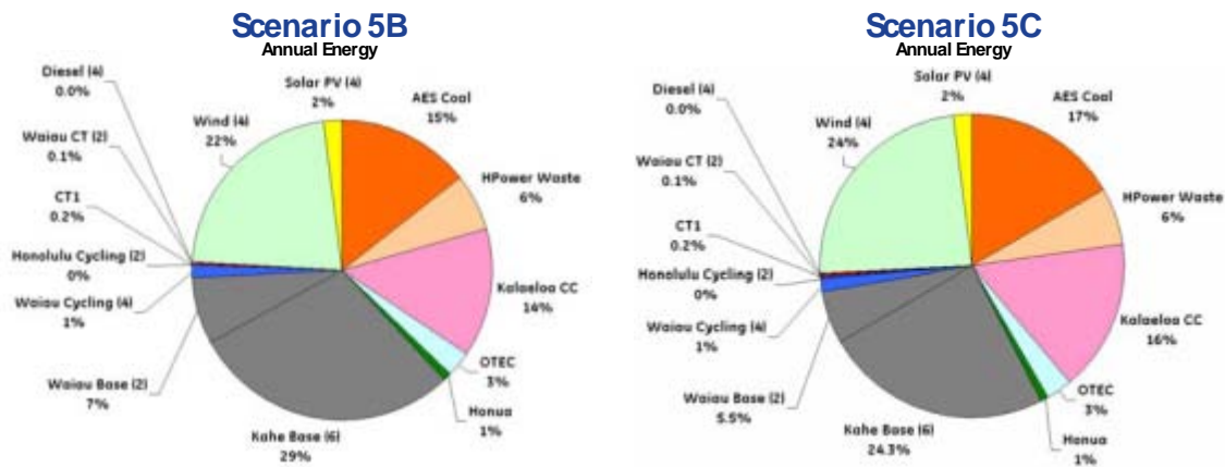
Figure 7-1. Scenario 5C: Annual energy production by unit type
