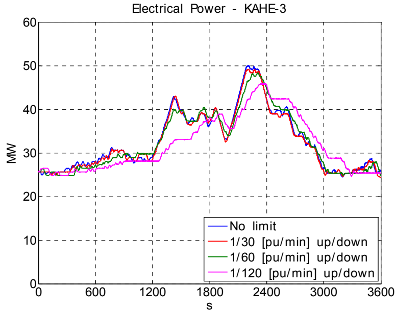
Figure 8-41. Kahe 3 Unit response for various ramp-rate limits
