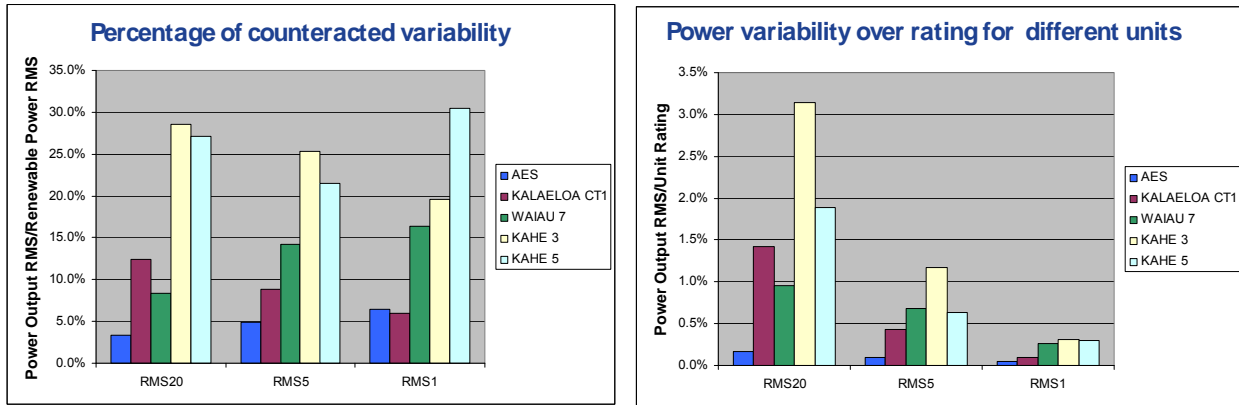
Figure 8-28. Hour 5795 Scenario 5F3 – Unit maneuvering. Left: figure: Percentage of variability counteracted by a specific unit. Right: figure: RMS power variability over the rating of each unit.
