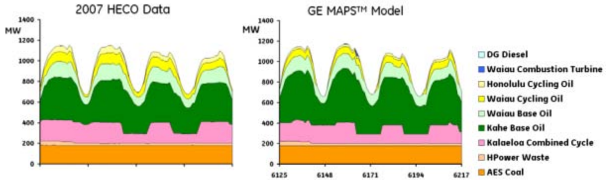
Figure 5-3 GE MAPS™ model results compared to historical hourly generation data for 4 days, starting September 13, 2007 and ending September 16, 2007
