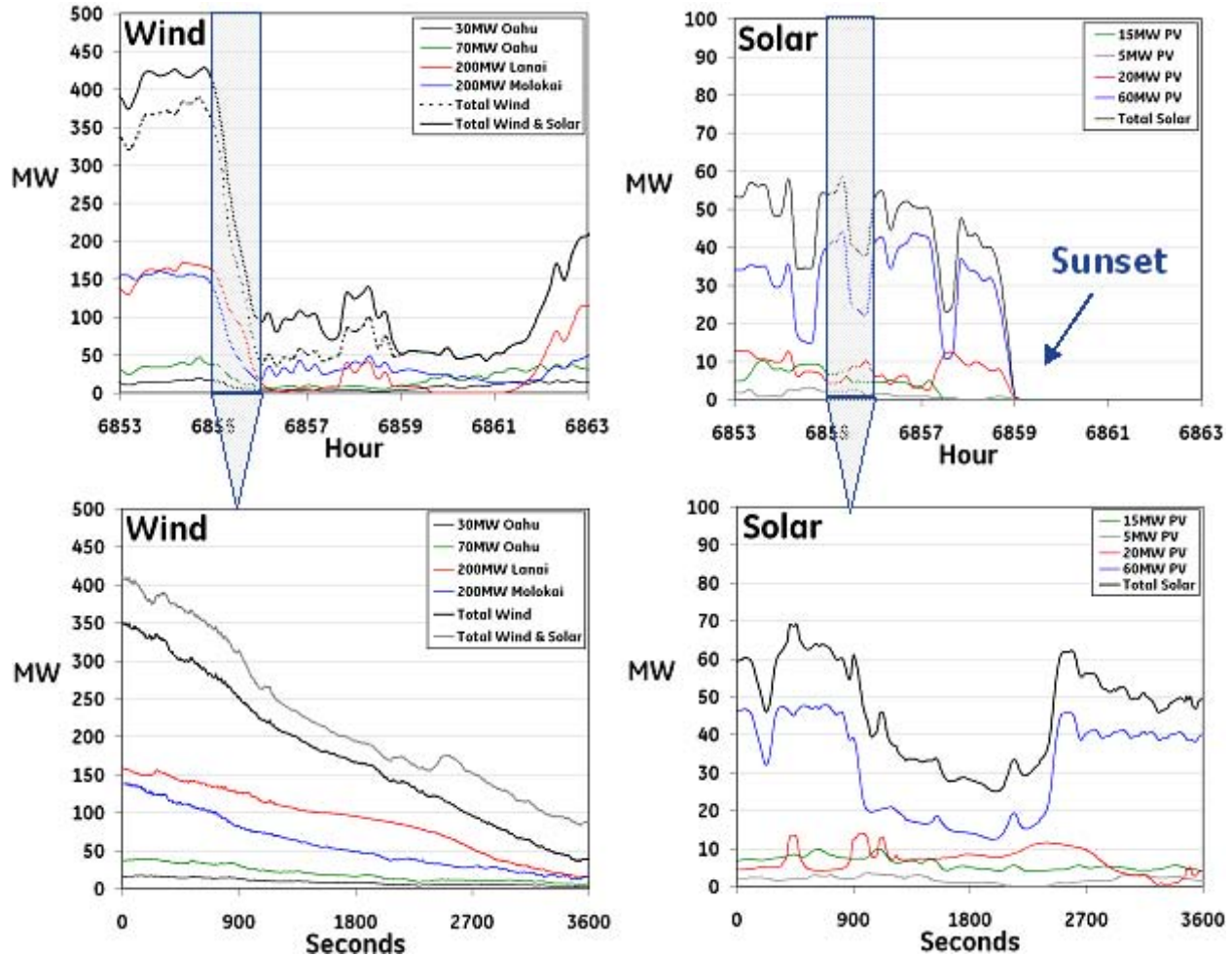
Figure 8-4. Drop in wind and solar power during the Hour 6855
