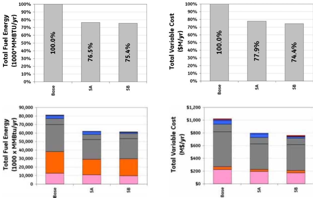
Figure 6-18. Scenario 5. Fuel energy and total variable cost of operation
