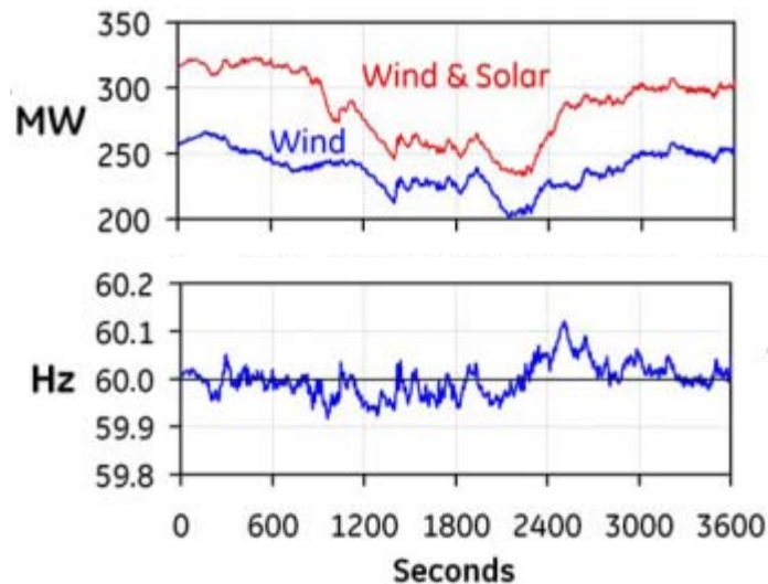
Figure 1-13. Impact of large swings in wind power on system frequency with the proposed thermal unit ramp rate capability and droop response (Scenario 5)
