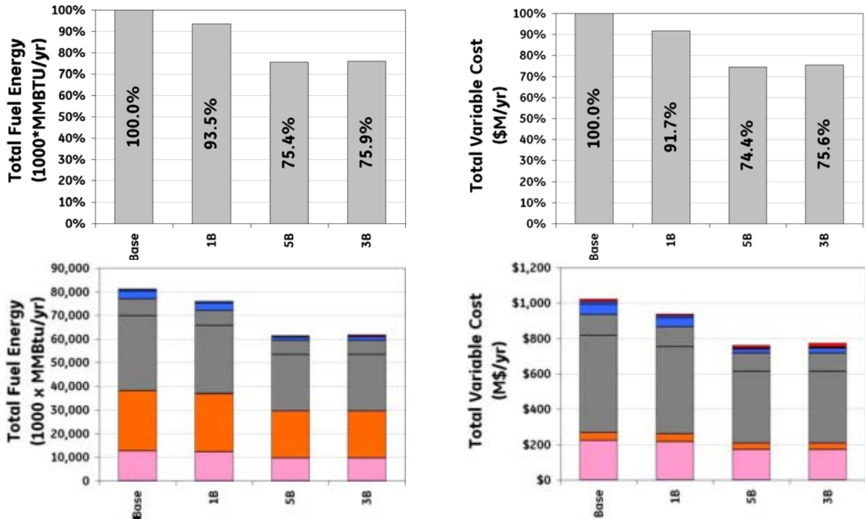
Figure 6-21. Scenario 3. Fuel energy and total annual variable cost of operation
