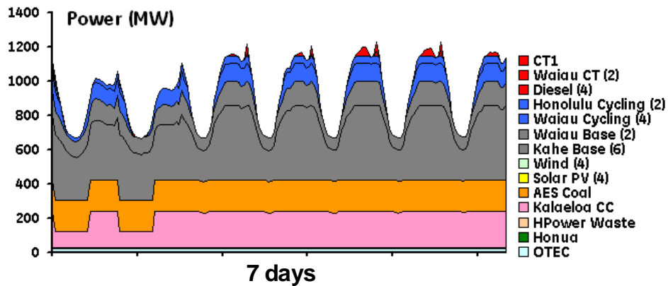
Figure 1-3. An example of operation for the Baseline 2014 Oahu power system
