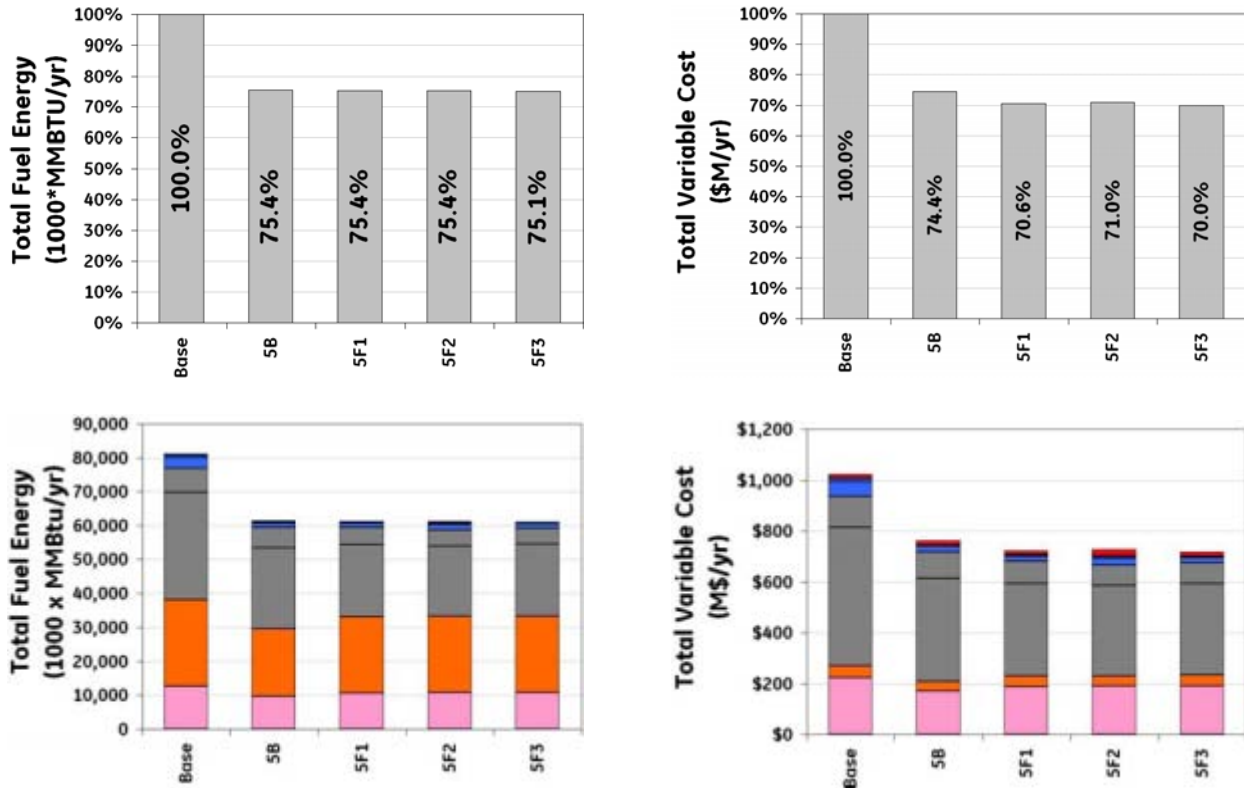
Figure 7-17. Scenario 5F3: Fuel energy and total variable cost of operation
