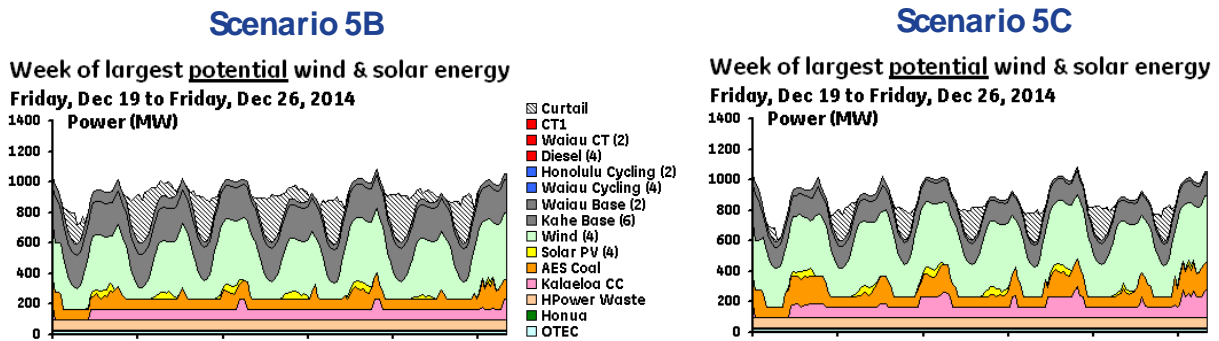
Figure 7-2. Scenario 5B and 5C. The week of Dec 19, 2014, in the future study year. This week exhibited the highest available wind energy.
