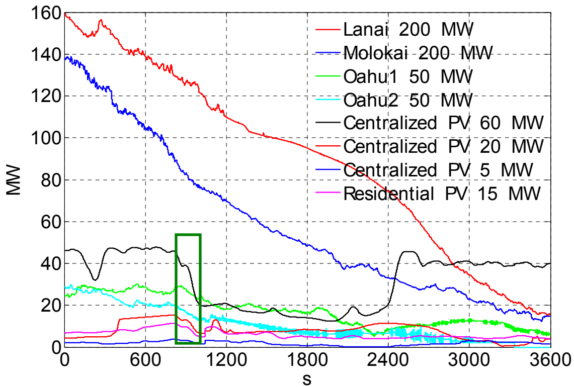
Figure 8-6. Wind power variability with modified solar for Hour 6855
