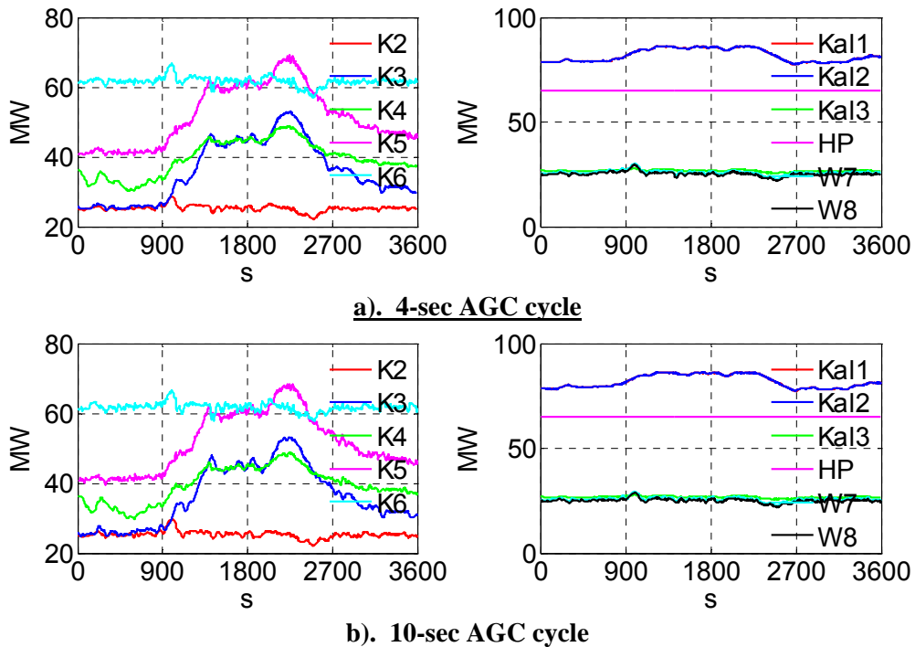
Figure 8-33. Hour 5795 Scenario 5F3 - Generating Unit Response
