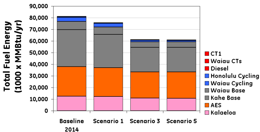
Figure 1-7. Total annual fuel consumption by Scenario.
