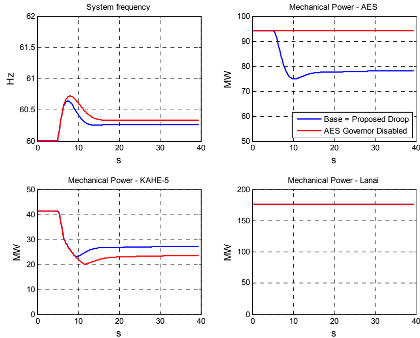
Figure 8-44: PSLF transient simulation result for 80 MW load rejection (Sc 5F3, AES governor sensitivity)
