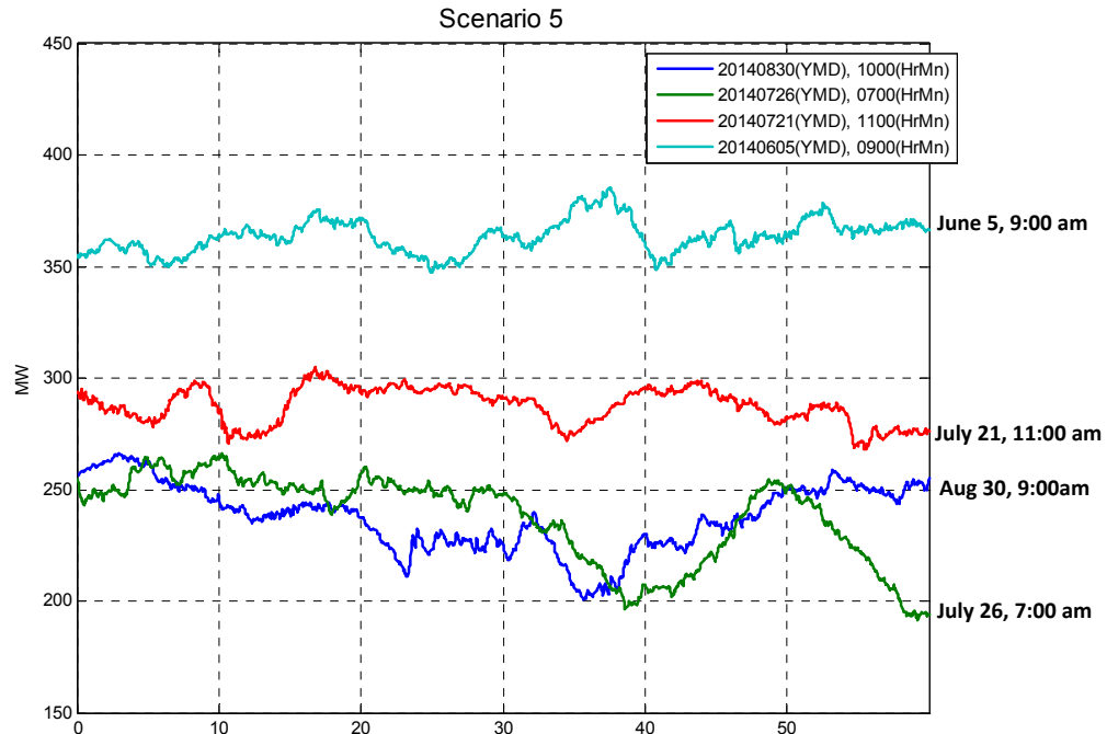
Figure 8-22. Total wind power trace for most severe hours in both 5 minute and 10 minute screening for Scenario 5 (x-axis in minutes for one hour)
