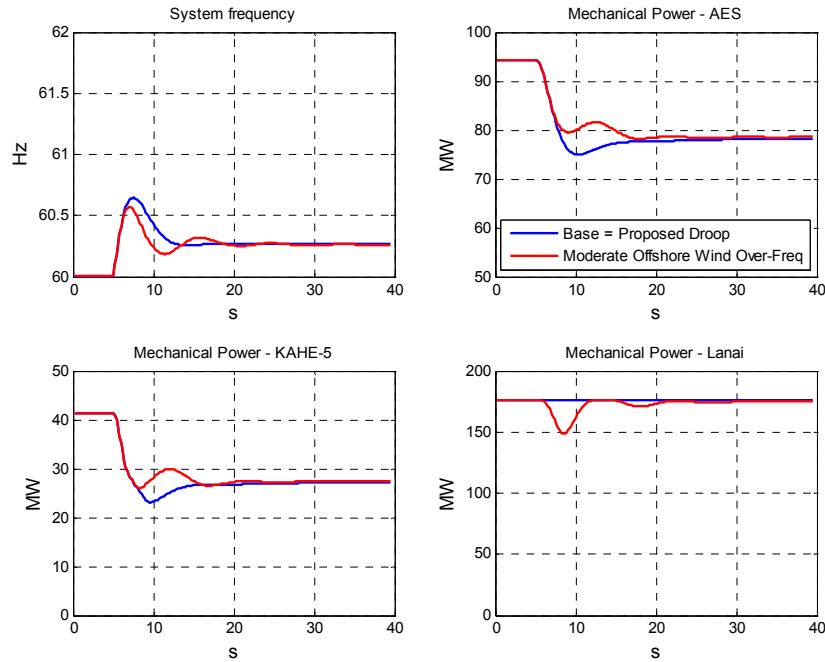
Figure 8-45: PSLF transient simulation result for 80 MW load rejection (Sc 5F3, moderate offshore wind plants over frequency control)
