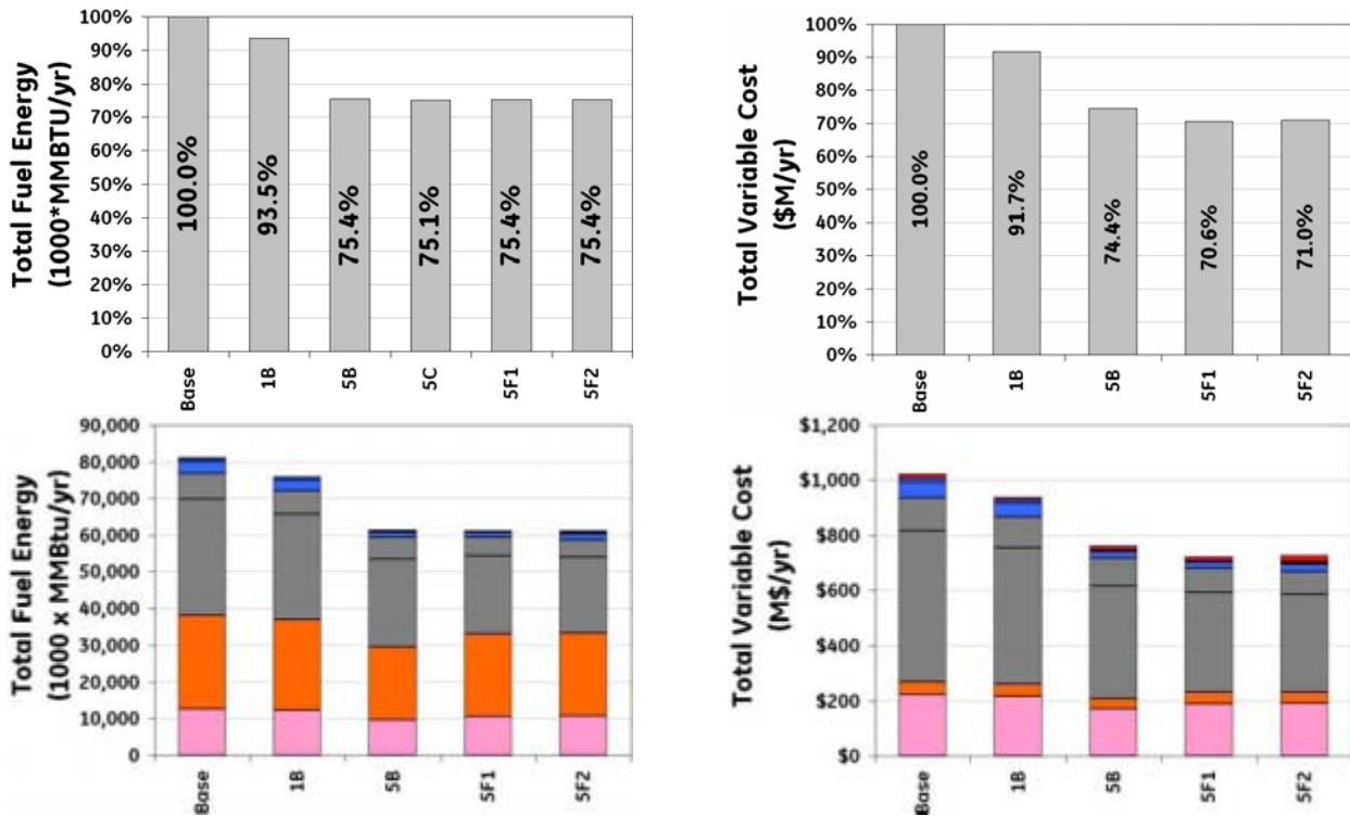
Figure 7-9. Scenario 5F2: Fuel energy and total variable cost of operation
