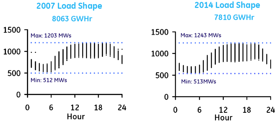
Figure 6-11. 2007 and 2014 load shapes
