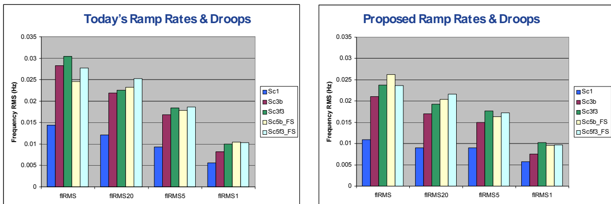
Figure 8-29. System frequency RMS across highly volatile wind events for each scenario. No solar variability and no governor response from AES were assumed.
