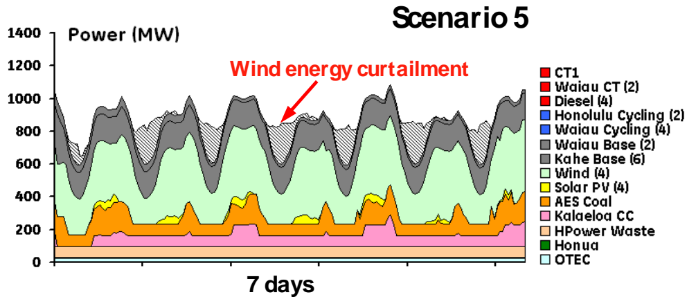
Figure 1-4. An example week of operation for the Oahu power system with 500 MW of wind power and 100 MW of solar power (Scenario 5)
