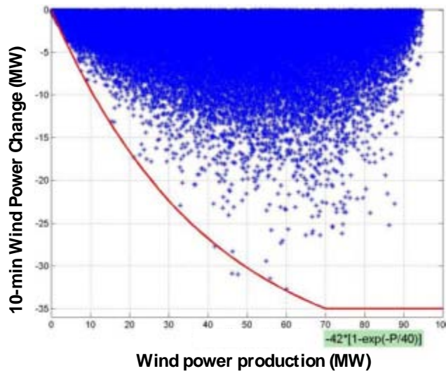
Figure 6-14. The regulating reserve requirement for Scenario 1 based on wind power production [ \text{func}(W) ]
