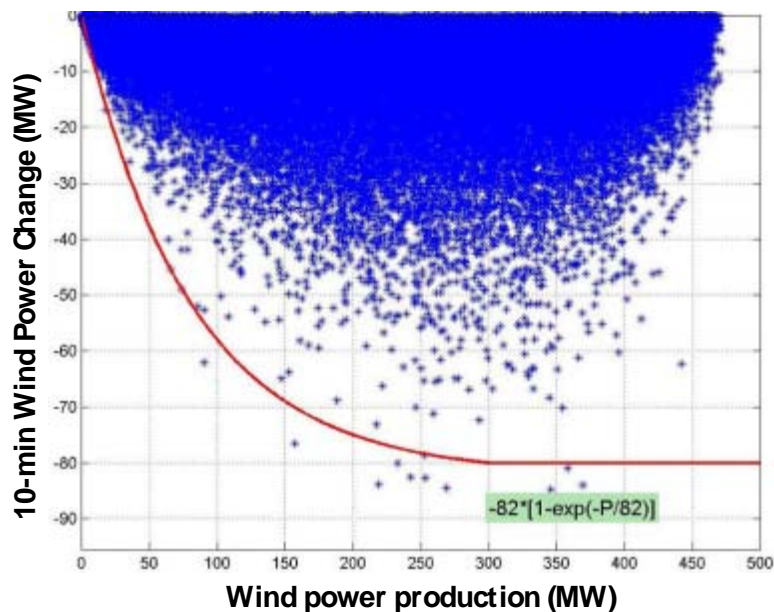
Figure 7-26. Total wind power changes over 10 minute intervals in Scenario 5 (two years of simulated wind power data from AWS Truepower).
