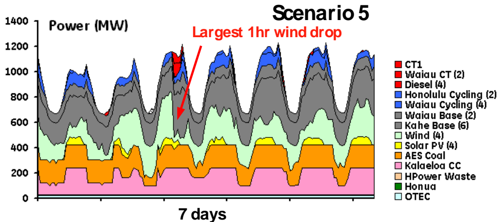
Figure 8-1. Hour 6855. Production cost dispatch and commitment for Scenario 5B
