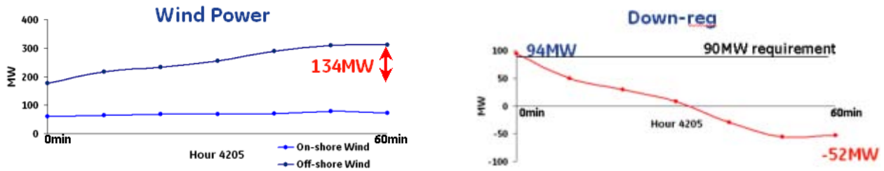
Figure 8-17. A challenging 60 minute event in Scenario 5F3
