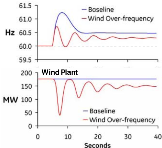
Figure 1-15. 140 MW load rejection event in Scenario 5 with future thermal unit droop characteristics, with and without wind turbine over-frequency control (3% droop / 30 mHz deadband).
