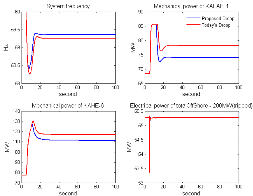
Figure 8-51: Transient simulation result for 200 MW cable trip for scenario 3F3. Sensitivity to thermal unit droop. Proposed droop (blue) and today's droop (red)
