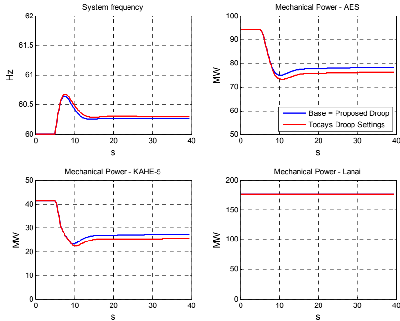
Figure 8-43: PSLF transient simulation result for 80 MW load rejection (Sc 5F3, thermal unit droop)
