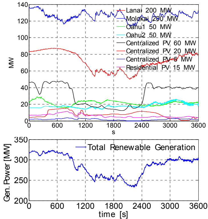
Figure 8-31. Wind and Solar Power variability – Hour 5795, Scenario 5F3
