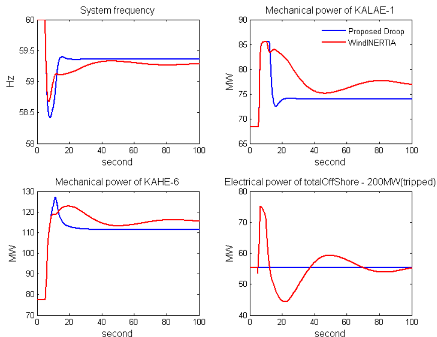
Figure 8-52: Transient simulation result for 200 MW cable trip for scenario 3F3. Sensitivity to WindINERTIA. Base case (blue) and WindINERTIA case (red)
