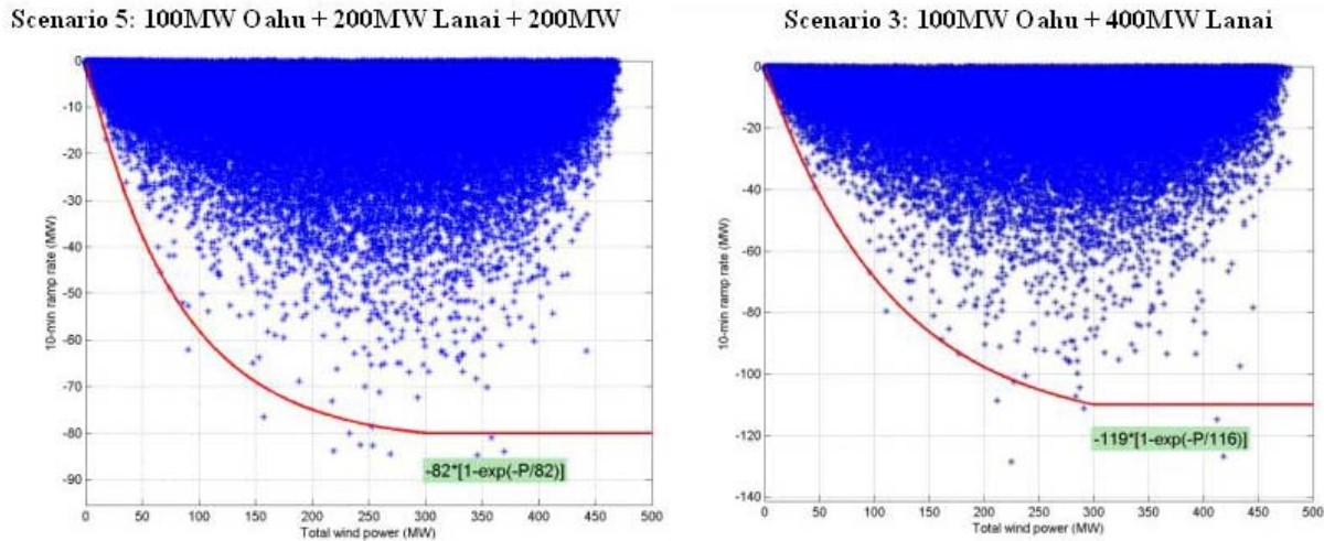
Figure 6-2 Ten minute wind power changes, based on two years of data, for Scenario 5 and Scenario 3
