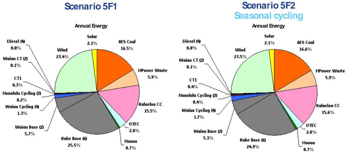
Figure 7-6. Scenario 5F2. Annual energy production by unit type
