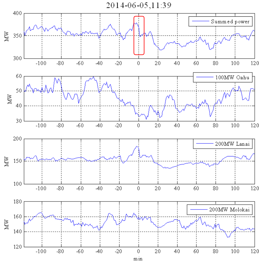
Figure 6-3 The largest 1 minute wind power drop for 100 MW Oahu + 200 MW Molokai + 200 MW Lanai (Scenario 5, excluding PV) from 2007 and 2008 modeled wind power data.
