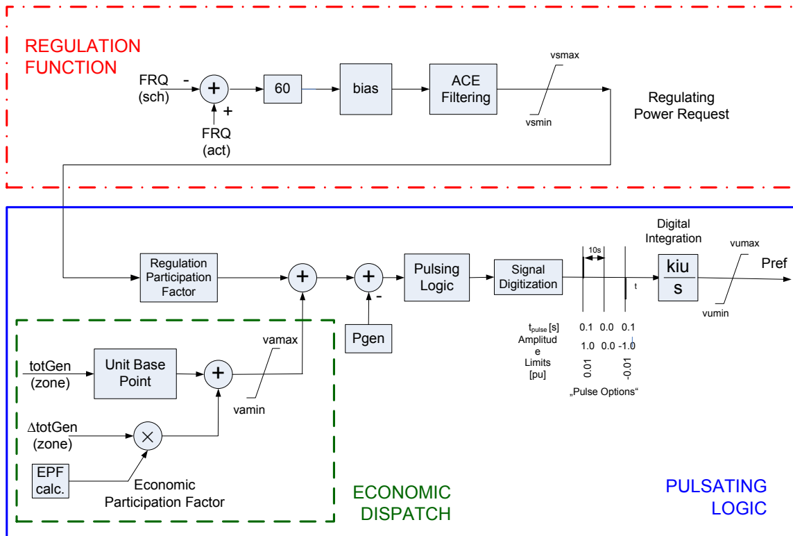
Figure 5-6 AGC model block diagram in normal operation mode
