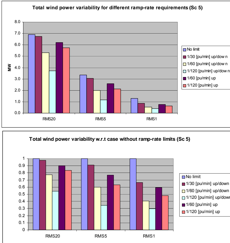
Figure 8-38. Effect of ramp rate limits at wind plants
