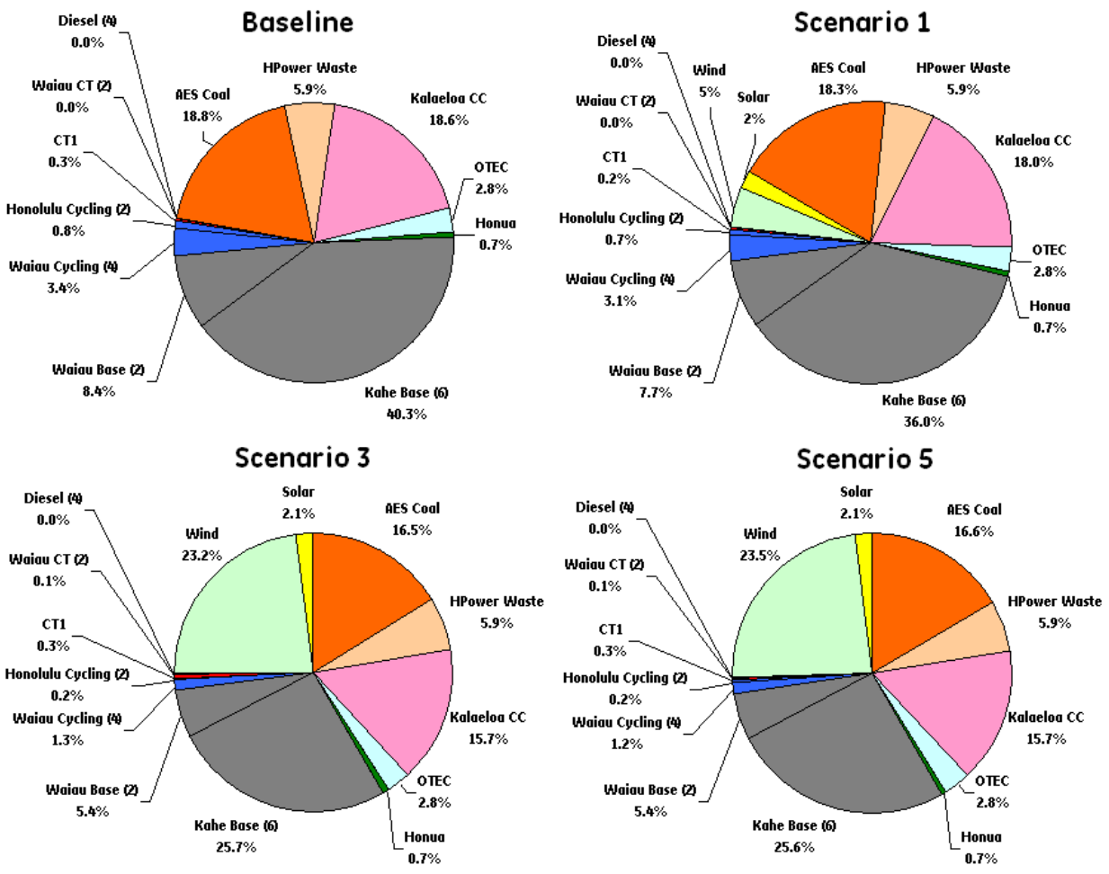
Figure 1-6. Share of annual energy production by fuel and unit type for each scenario.
