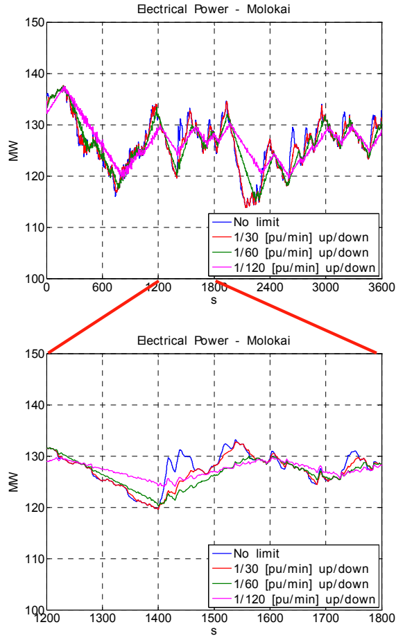
Figure 8-37. Ramp rate limits applied to 200 MW Molokai wind plant (top: one-hour, bottom: 10 minute zoom)
