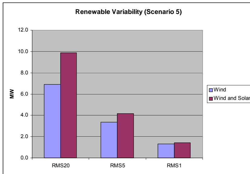
Figure 8-24. Wind and solar variability for selected outliers
