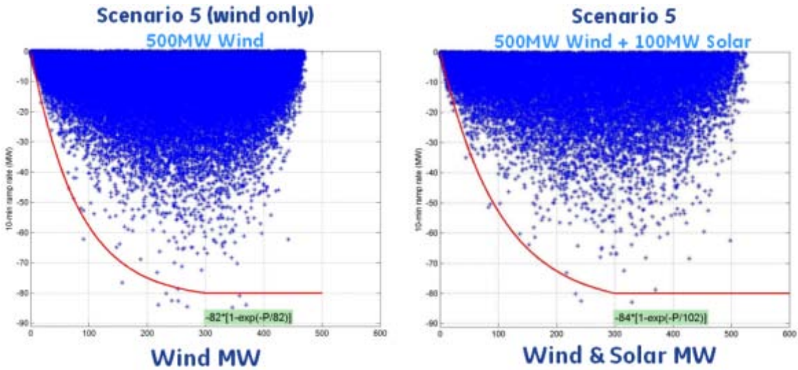
Figure 7-11. Regulating reserve function based on wind and solar forecast
