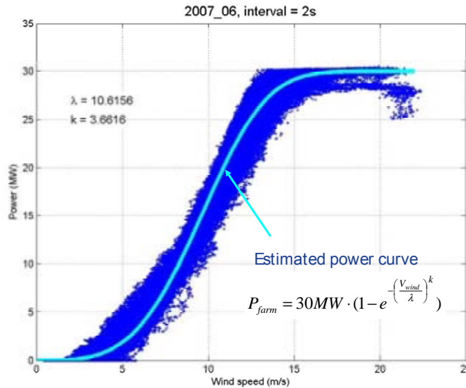
Figure 6-1 Kaheawa Wind Plant, Maui historical (2007 June) data Note that curtailment periods were removed from the historical data.
