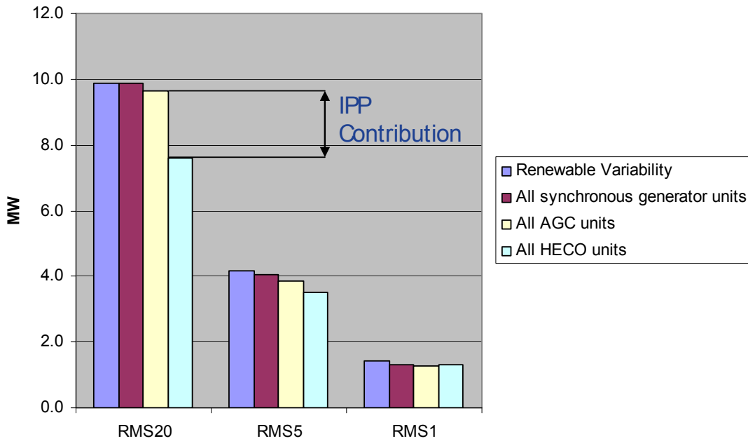
Figure 8-27. Hour 5795 Scenario 5F3 - Variability Sharing among Units (proposed ramp rates)
