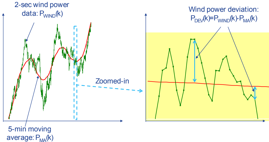
Figure 8-21. RMS calculation of high frequency wind turbulence
