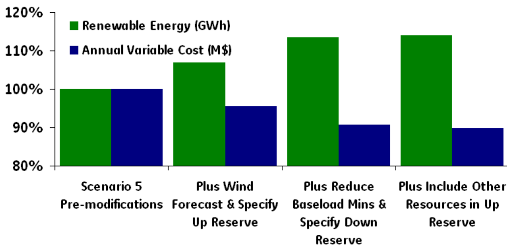
Figure 7-25. Scenario 5. Reduction in variable cost and increase in wind and solar energy delivered for staged strategies.
