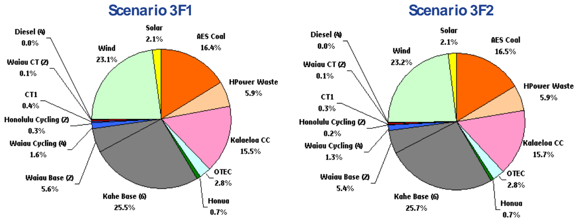
Figure 7-21. Scenario 3F2. Annual energy production by unit type
