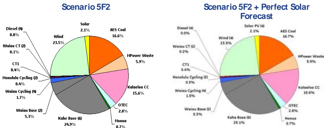
Figure 7-10. Scenario 5F2 with no solar forecast (left) and a perfect solar forecast (right). Annual energy production by unit type
