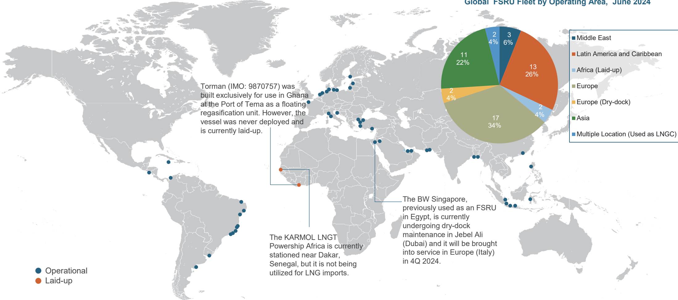
Global FSRU Fleet by Operating Area, June 2024
