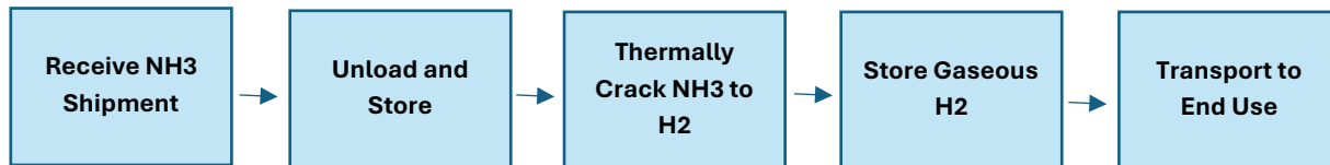
Figure 21. Process for Ammonia Use as an Energy Carrier
