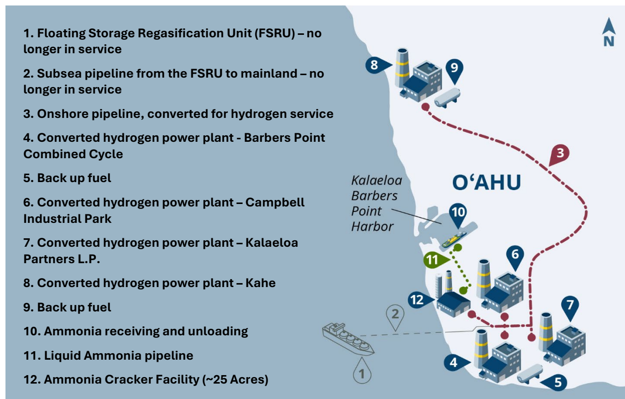
Figure 23. Ammonia Energy Concept for O'ahu
