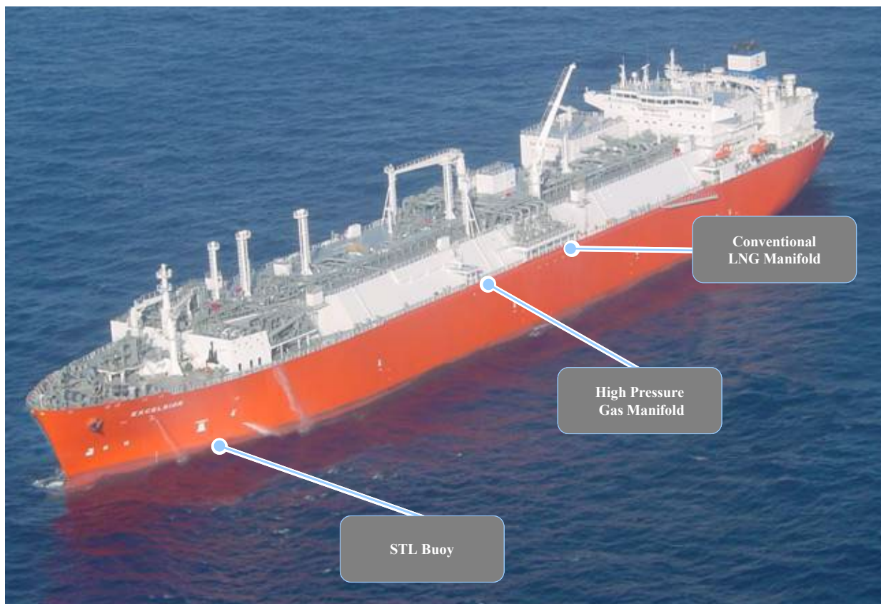
Figure 14. Overview of Gas Transfer Connections
