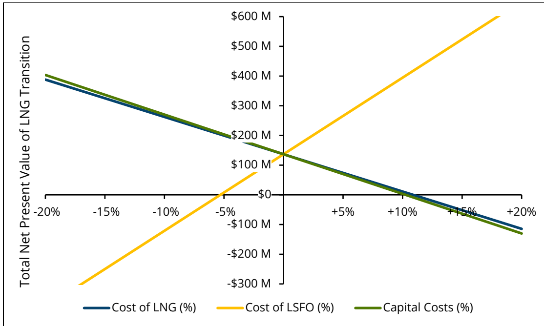
Figure 19. Sensitivity Analysis of Net Present Value of LNG Transition, Alternative 2A
