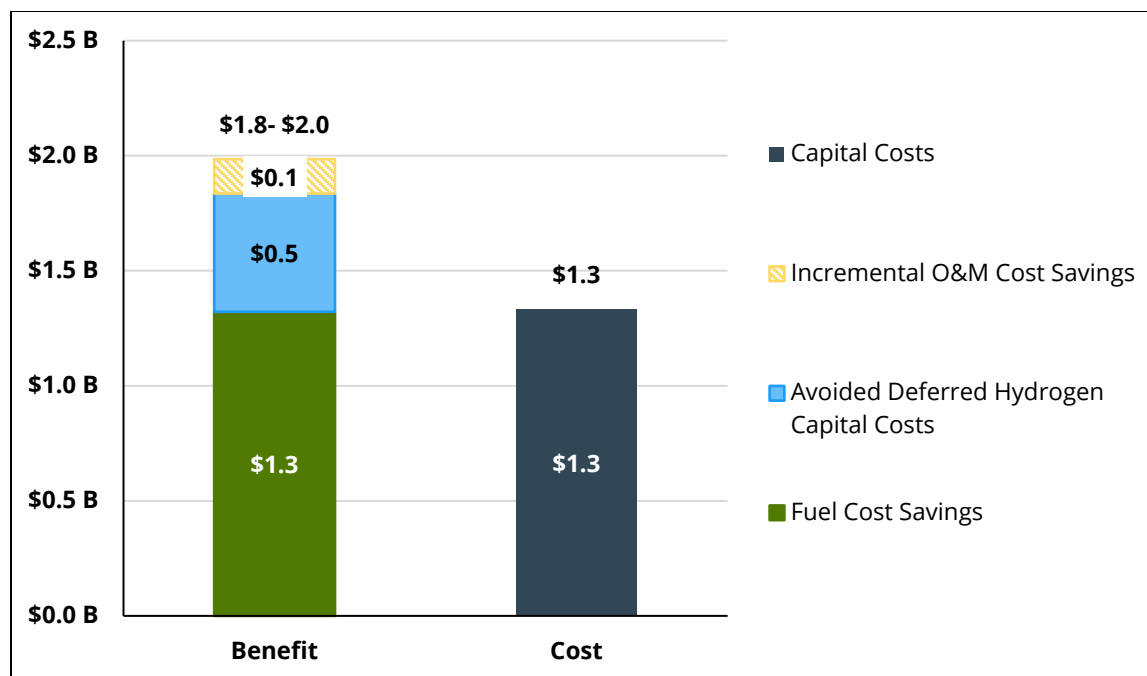
Figure 6. Alternative 1A net present value of LNG transition. Evaluation includes the re-use of LNG infrastructure after 2044 for renewable fuel.
