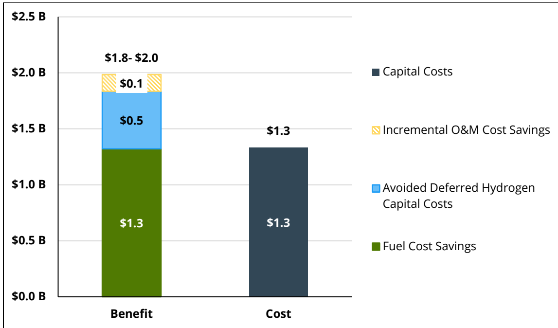
Figure 16. Alternative 1A net present value of LNG transition
