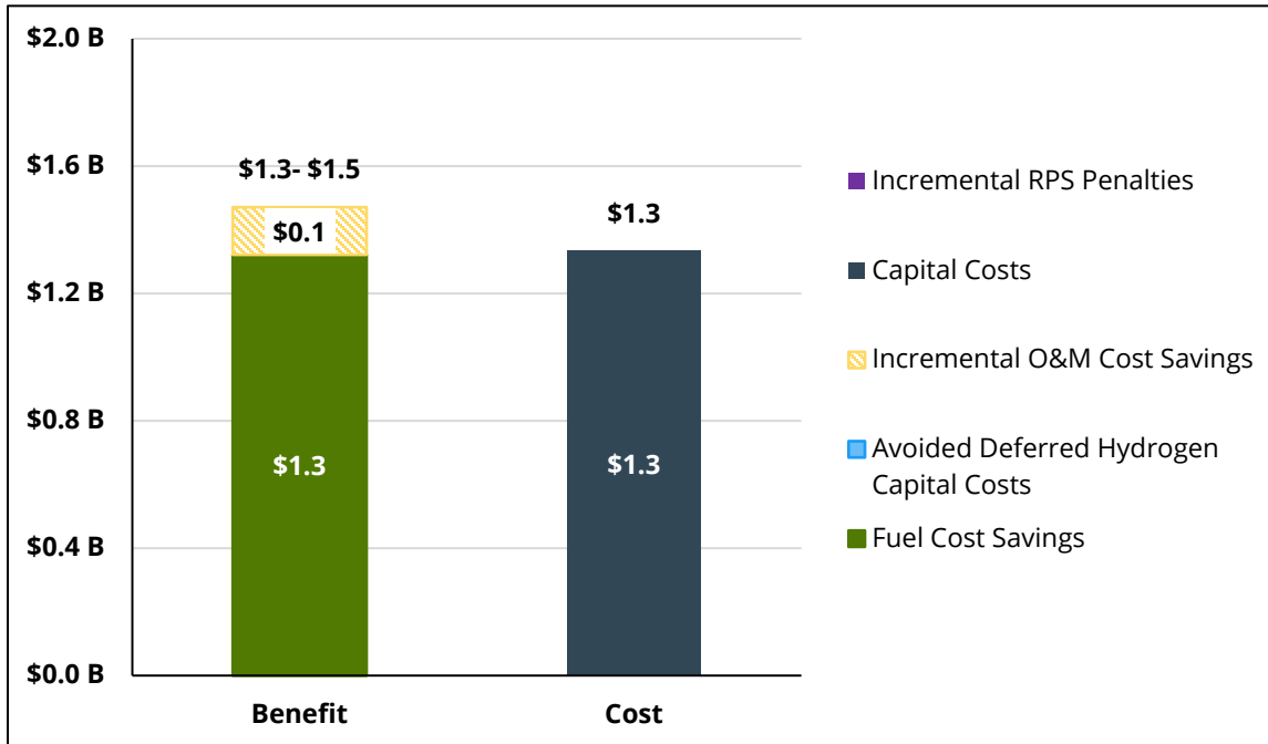
Figure 18. Alternative 2A net present value of LNG transition
