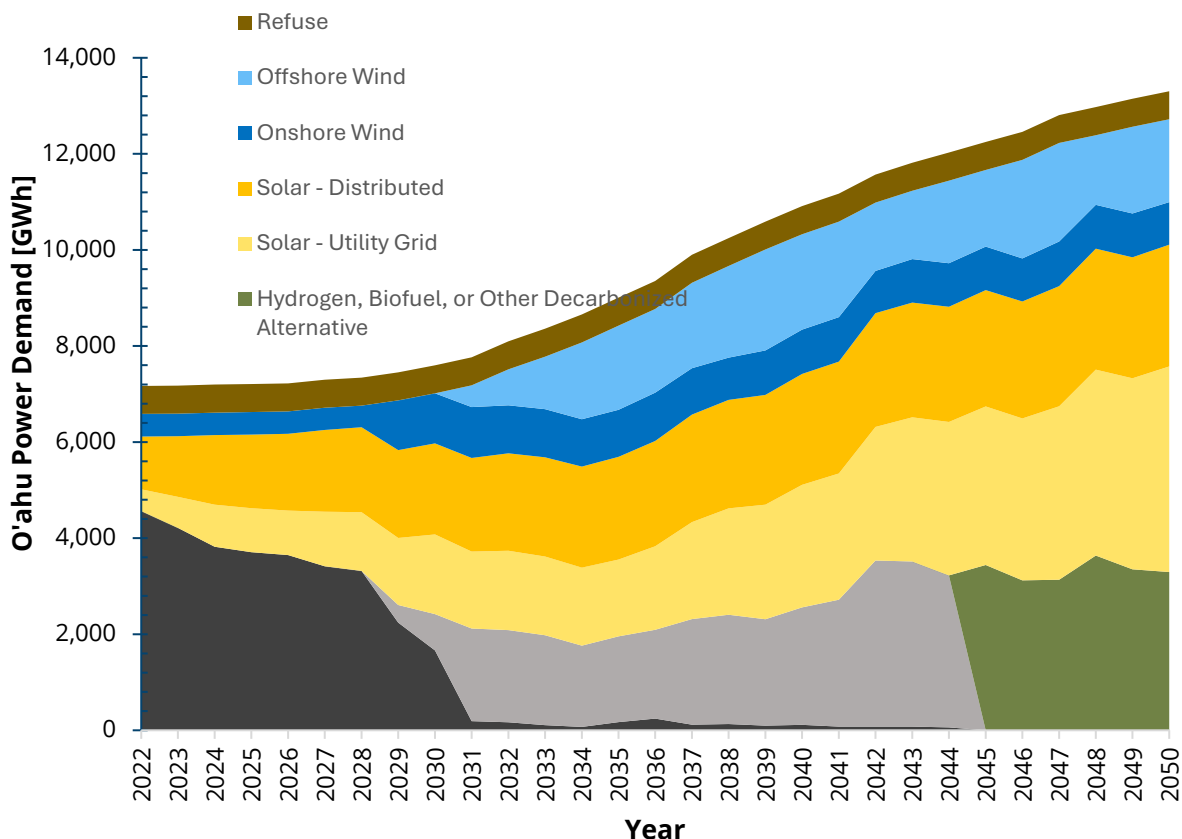
Figure 5. O'ahu forecasted future power demand and generation portfolio by technology type, based on conservative electrification forecast and capacity expansion modeling.
